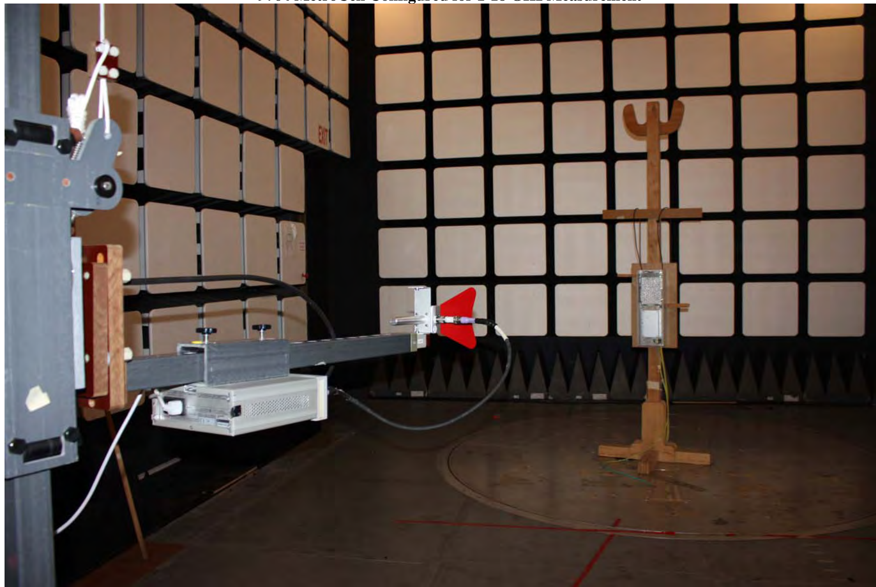
9764 MetroCell Configured for 1-18 GHz Measurement
