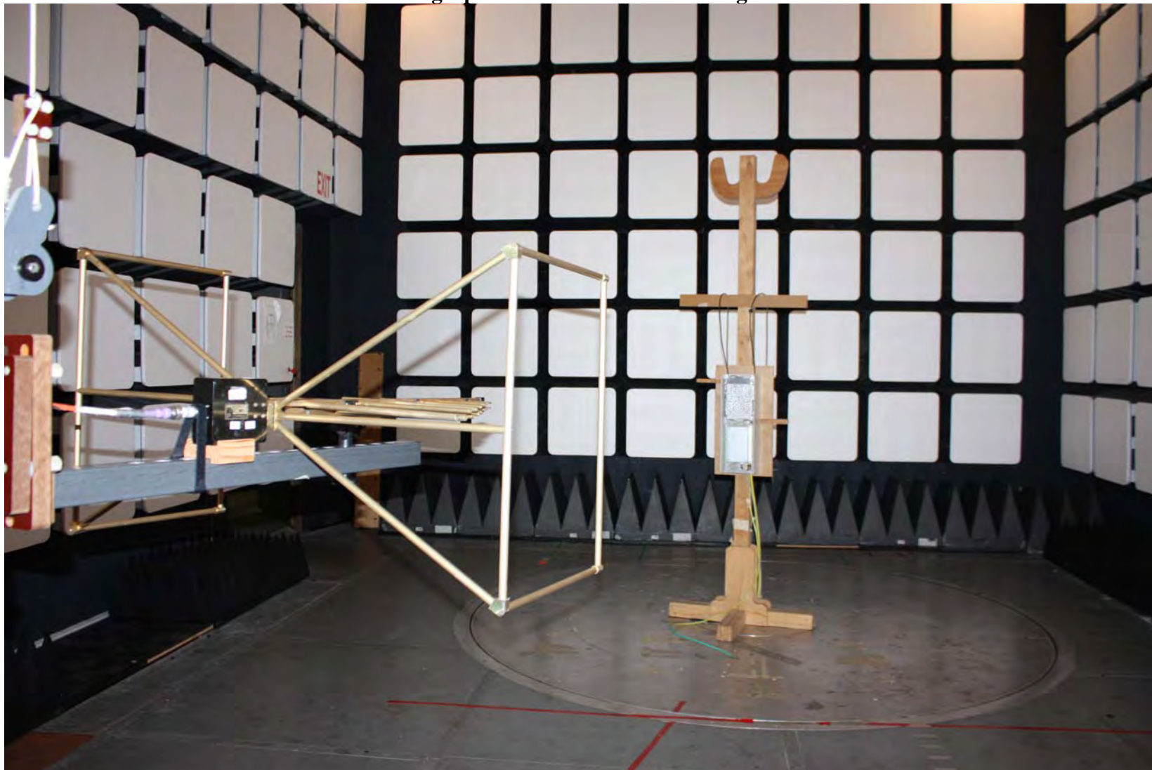
Radiated Emissions Test Photograph A 9764 MetroCell Configured for 30 MHz-1 GHz Measurement
