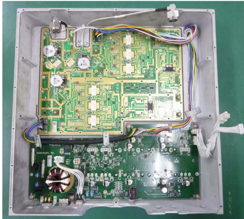
Photograph of PA and PS
