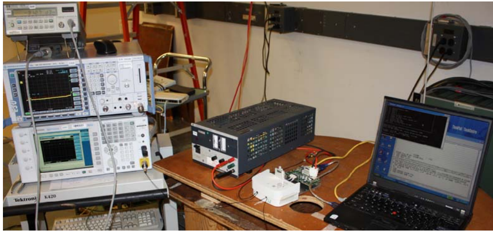
Figure 11.2 Setup Photo of Conducted Emissions Test at Antenna Ports.
