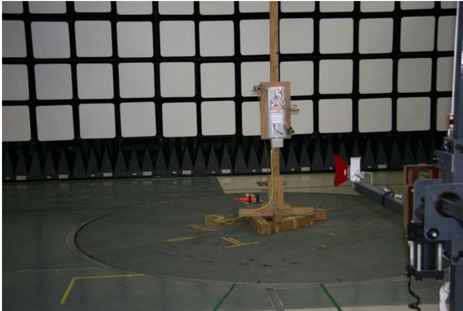
Figure 11.1 Setup Photo of Radiated Emissions Test
