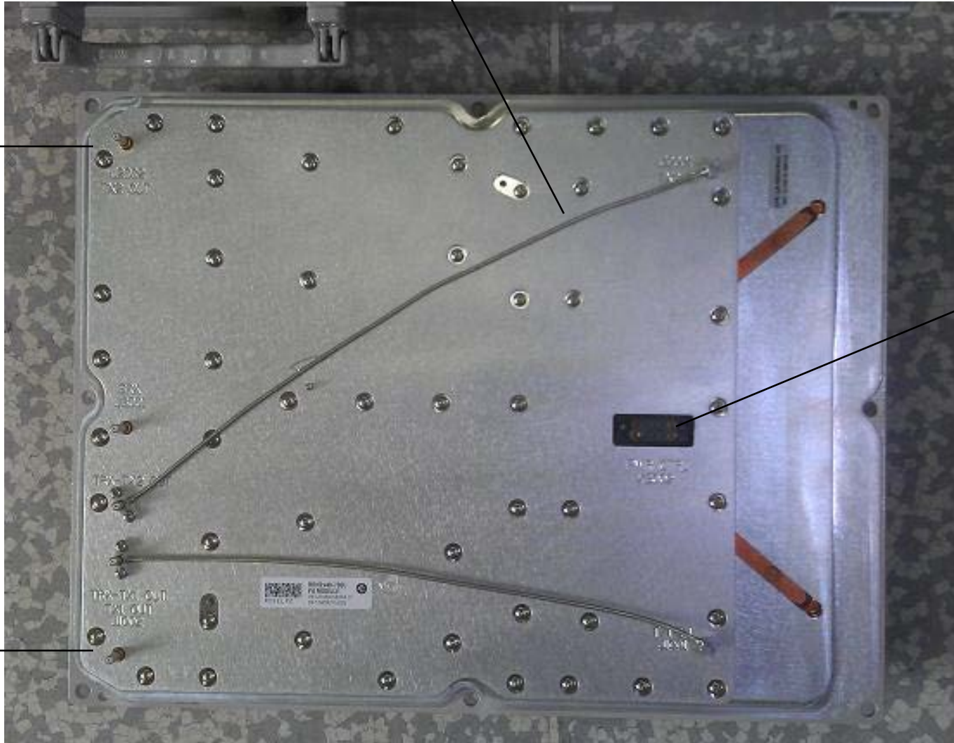
Figure 4 RRH2x40_07L-AT internal showing PA Module
