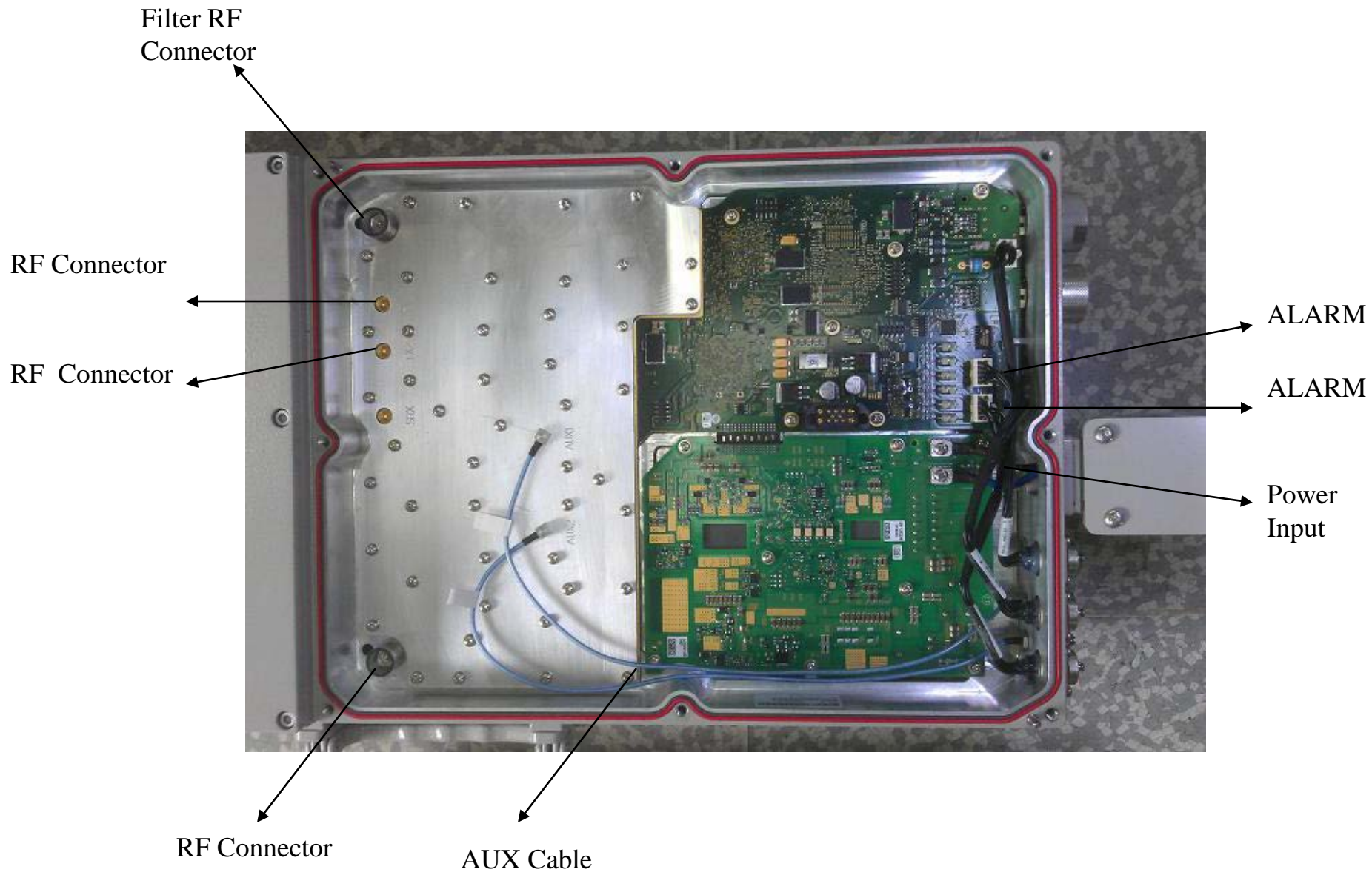
Figure 5 RRH2x40_07L-AT internal showing TRX and PSU
