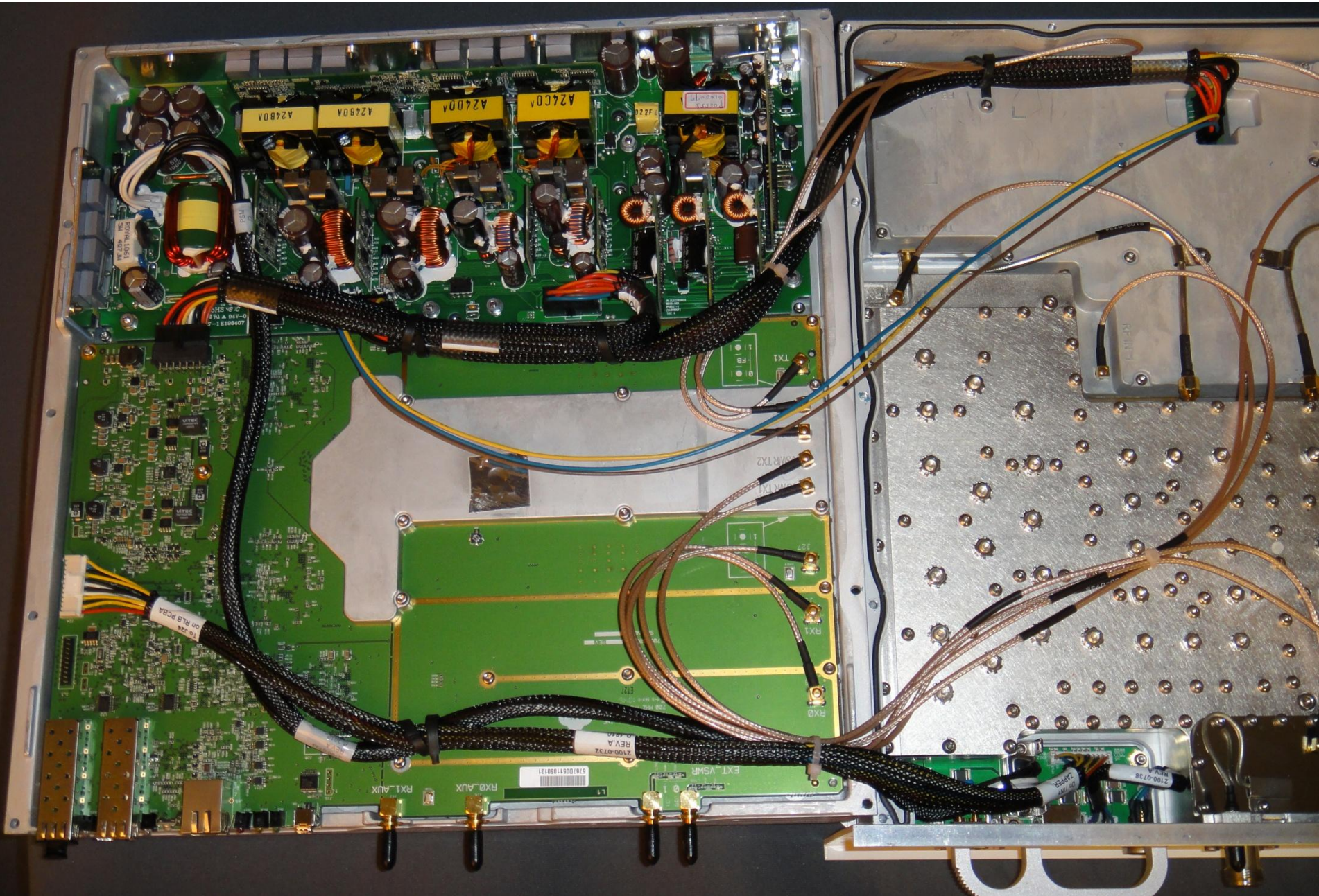
Photo 3 – Radio and Amplifier
