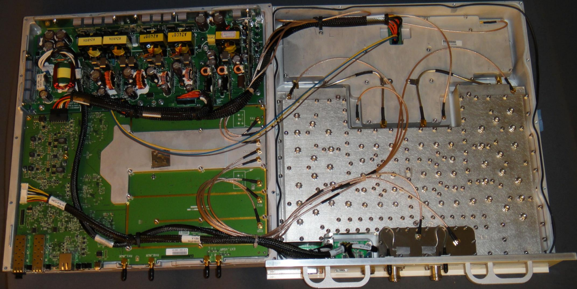
Photo 1: Full View Of Internals
