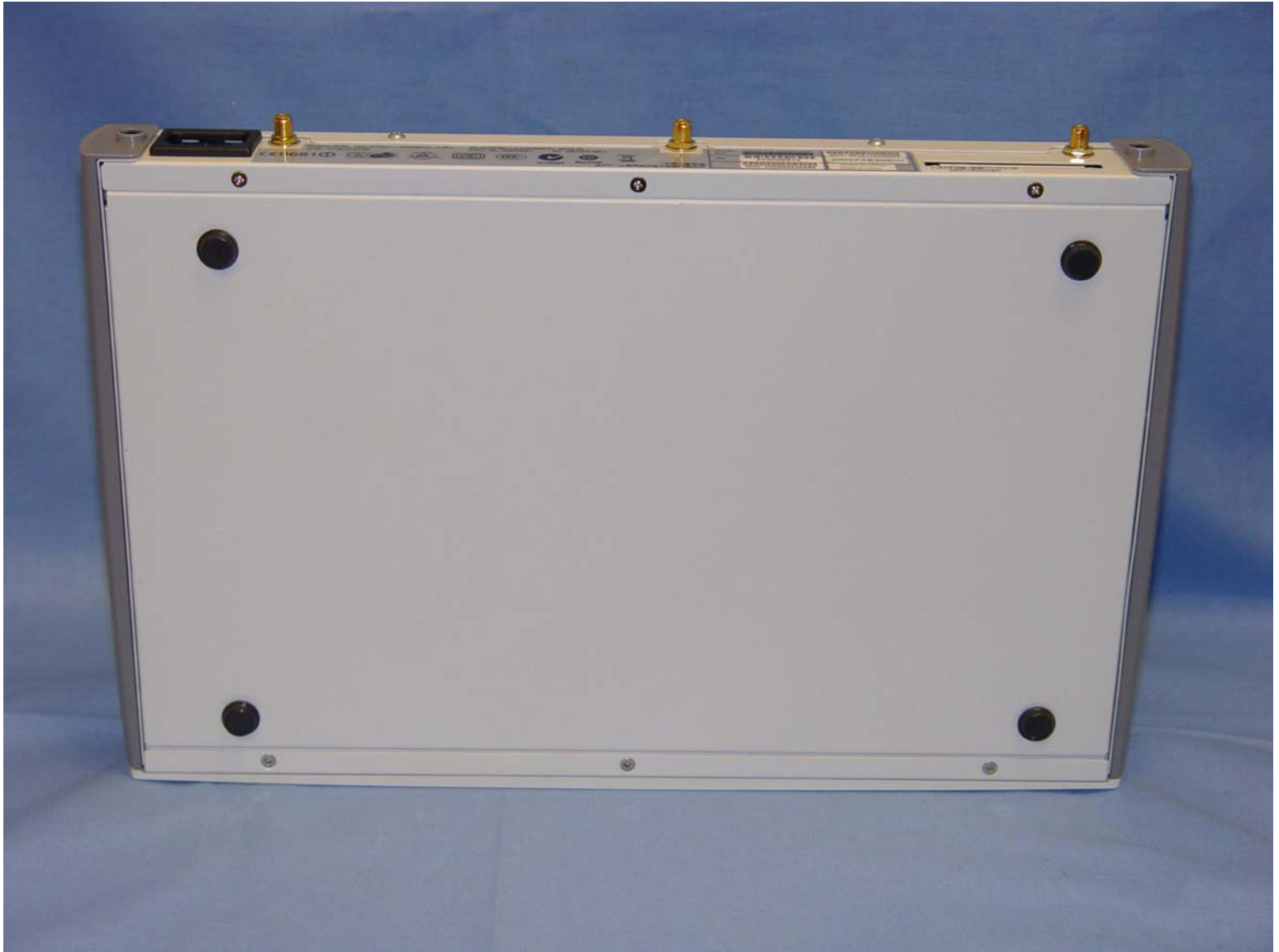
OAW-4306GW Bottom
