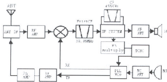
Fig1. Frequency configuration
