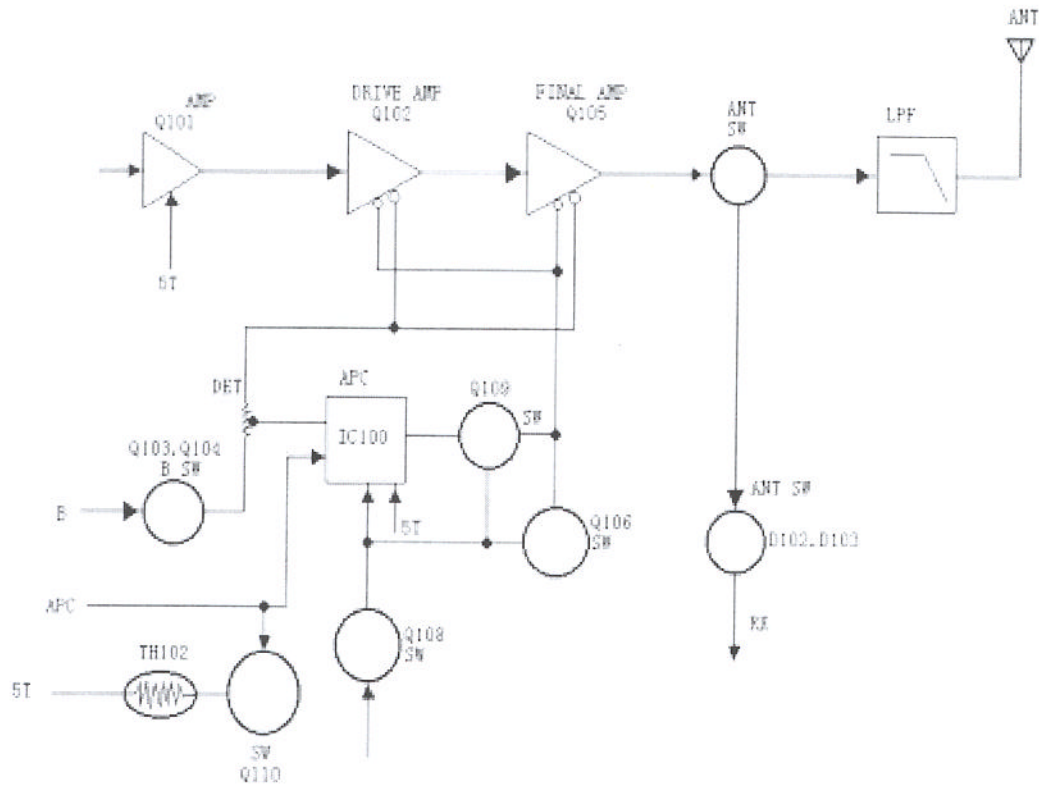
Fig. 7. APC system
