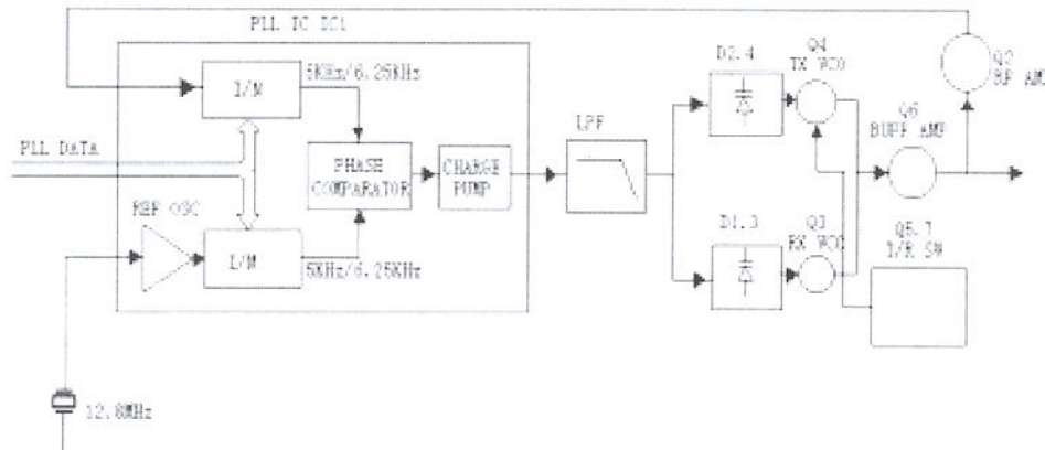
Fig. 4. PLL circuit
