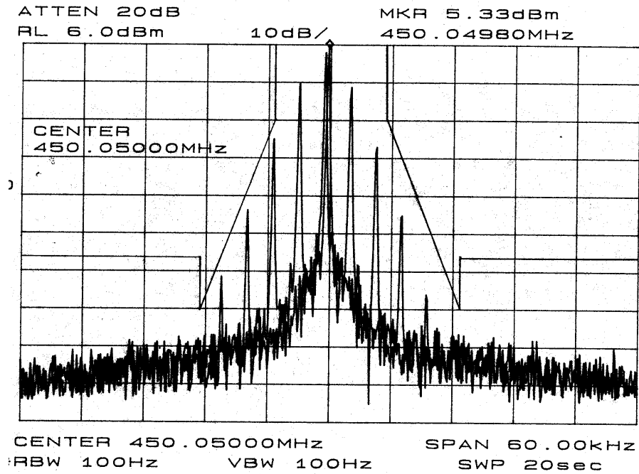
Graph 7 - Occupied Bandwidth in Narrow Band mode (12.5 KHz) at 450.050 MHz
