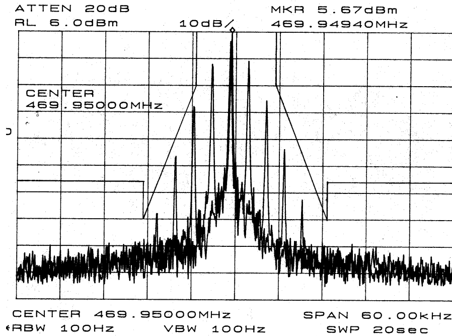
Graph 9 - Occupied Bandwidth in Narrow Band mode (12.5 KHz) at 469.950 MHz
