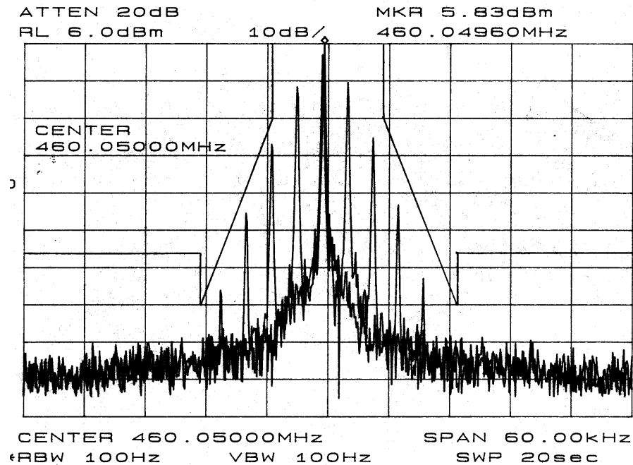
Graph 8 - Occupied Bandwidth in Narrow Band mode (12.5 KHz) at 460.050 MHz
