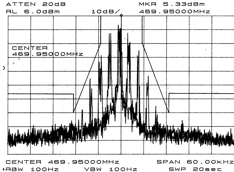
Graph 10 - Occupied Bandwidth with DCS in Narrow Band mode (12.5 KHz) at 469.950 MHz
