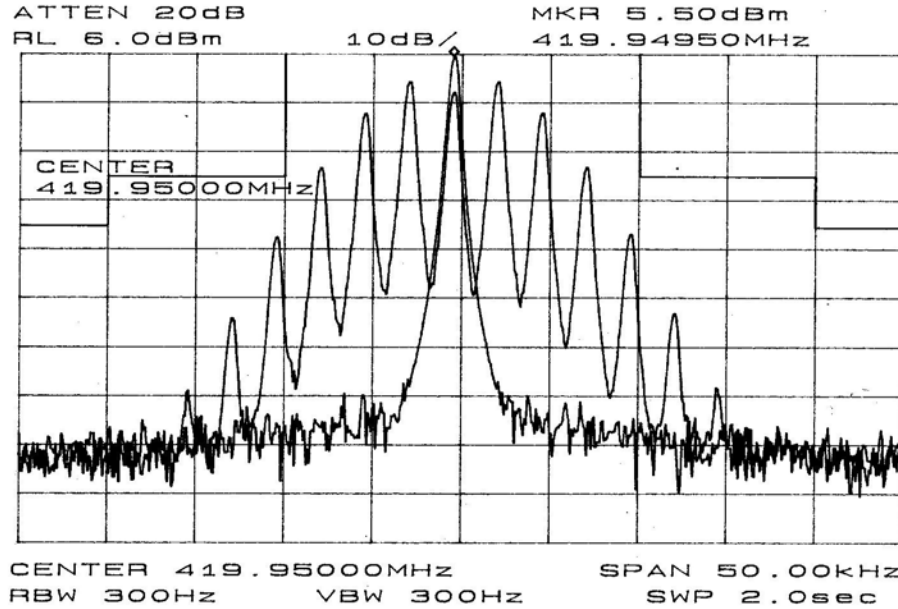
Occupied Bandwidth in Wide Band mode (25 KHz) at 419.950 MHz
