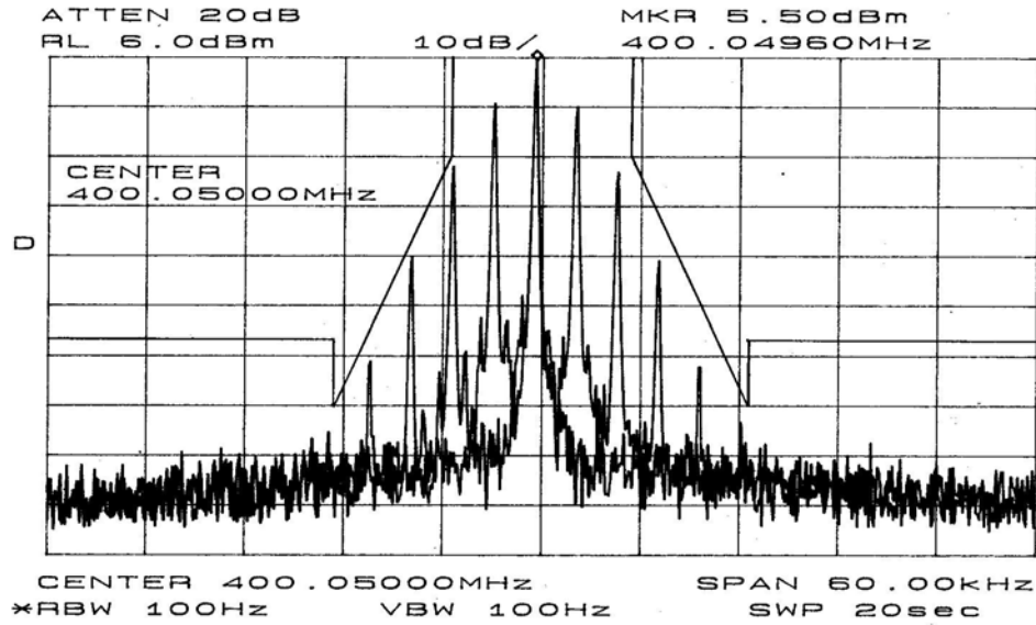
Occupied Bandwidth in Narrow Band mode (12.5 KHz) at 400.050 MHz
