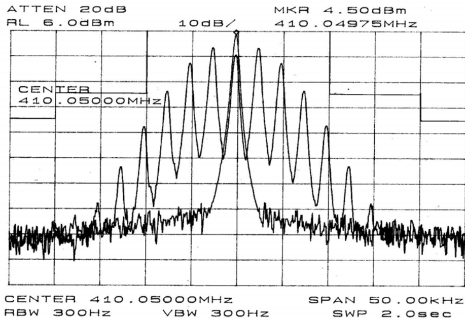
Occupied Bandwidth in Wide Band mode (25 KHz) at 410.050 MHz
