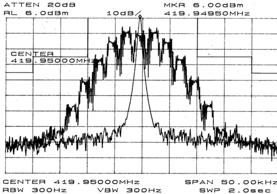
Occupied Bandwidth with DCS in Wide Band mode (25 KHz) at 419.950 MHz
