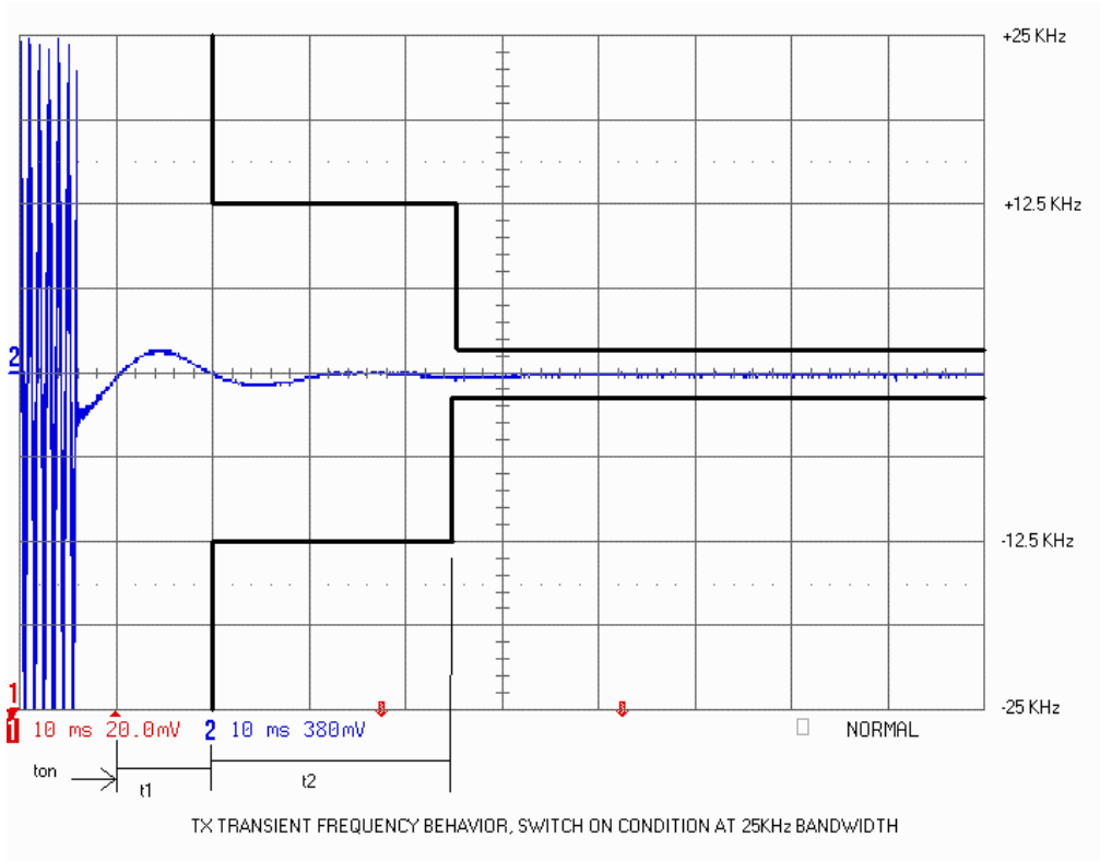
Transient Frequency Behavior Condition in Wide Band Mode (25 kHz)
