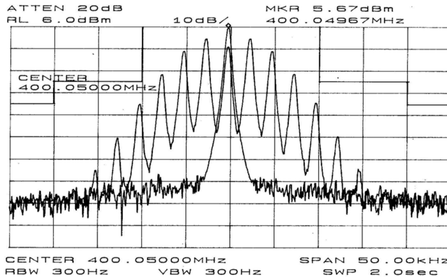
Occupied Bandwidth in Wide Band mode (25 KHz) at 400.050MHz
