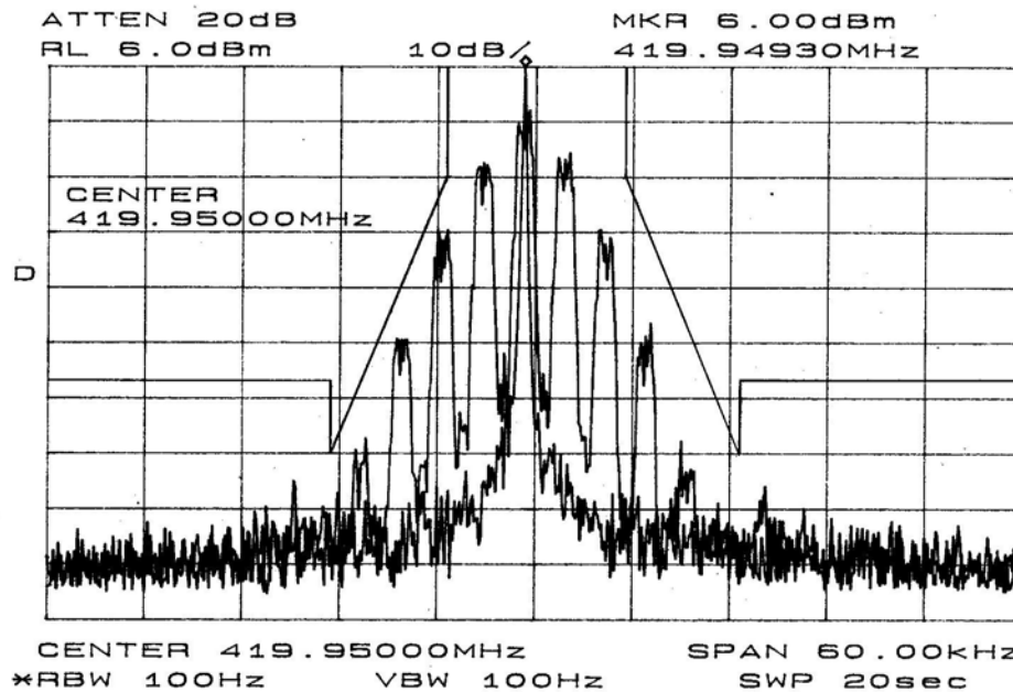
Occupied Bandwidth with DCS in Narrow Band mode (12.5 KHz) at 419.950 MHz
