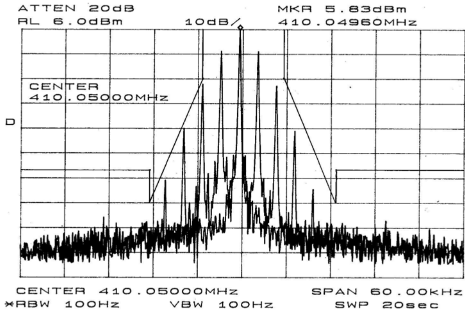
Occupied Bandwidth in Narrow Band mode (12.5 KHz) at 410.050 MHz
