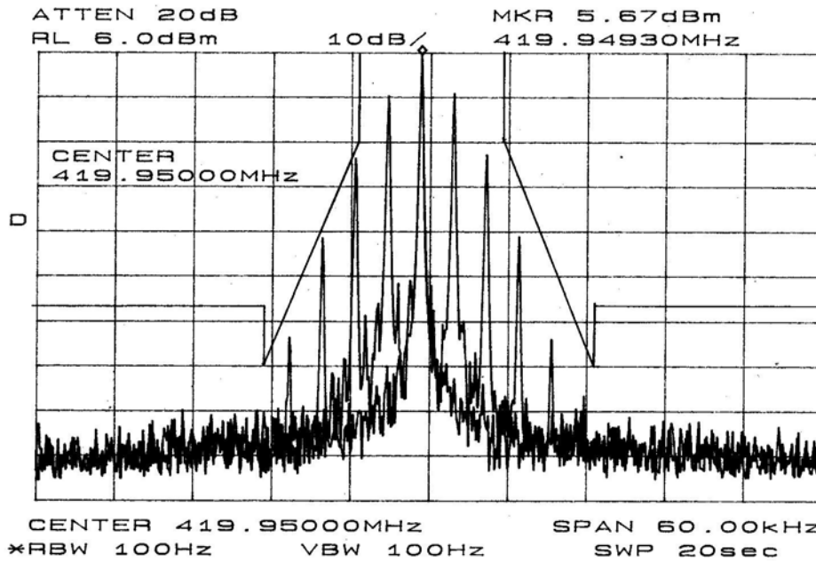
Occupied Bandwidth in Narrow Band mode (12.5 KHz) at 419.950 MHz
