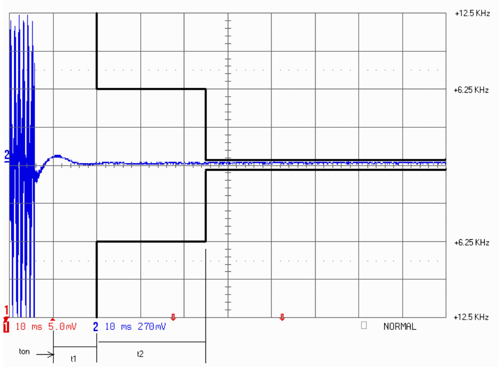
Transient Frequency Behavior Condition in Narrow Band Mode (12.5 kHz)
