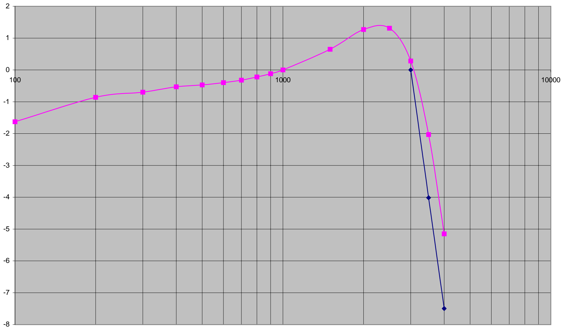
TC-268 TX Low-Pass Filter Response(Curve B)
