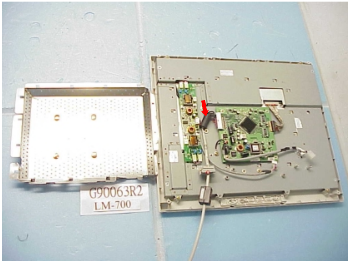
Figure 7 Internal View, M/N LM-700
