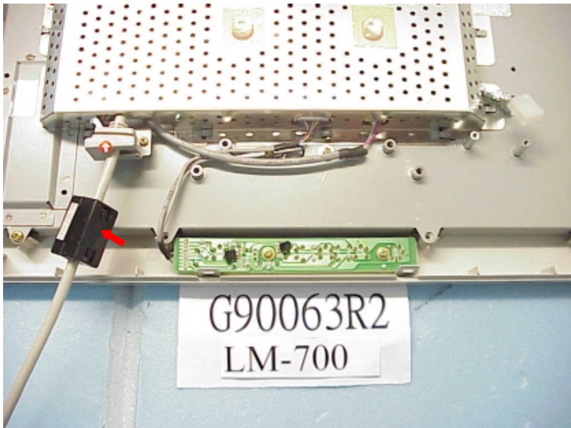
Figure 12 Internal View, M/N LM-700
