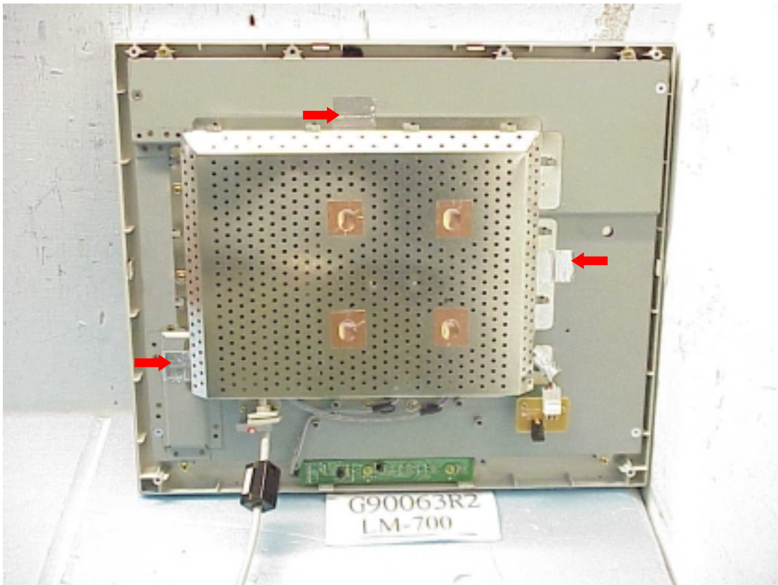
Figure 5 Internal View, M/N LM-700
