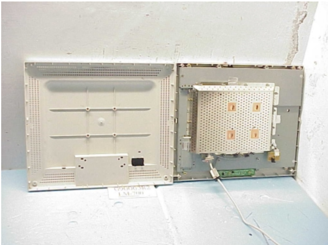
Figure 4 Internal View (Removed Back Cover), M/N LM-700
