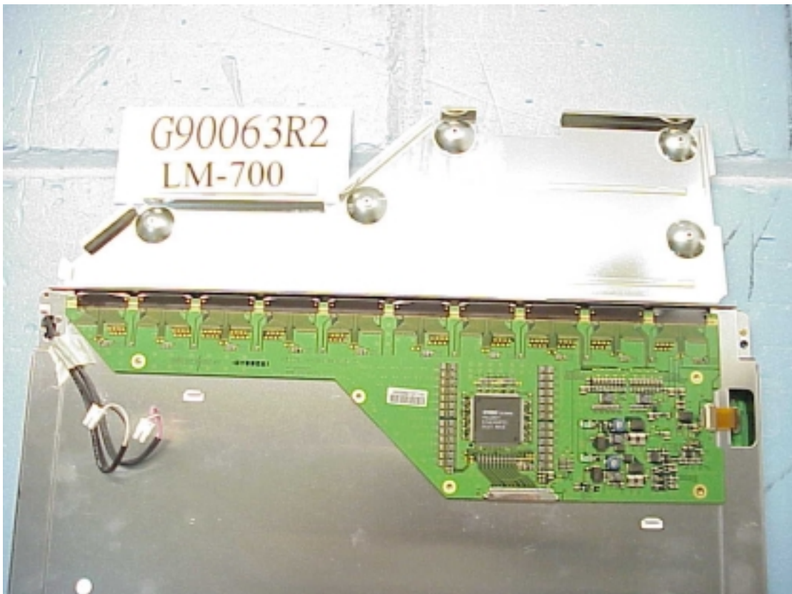
Figure 18 Control Board (Component Side) of LCD Panel, M/N LM-700
