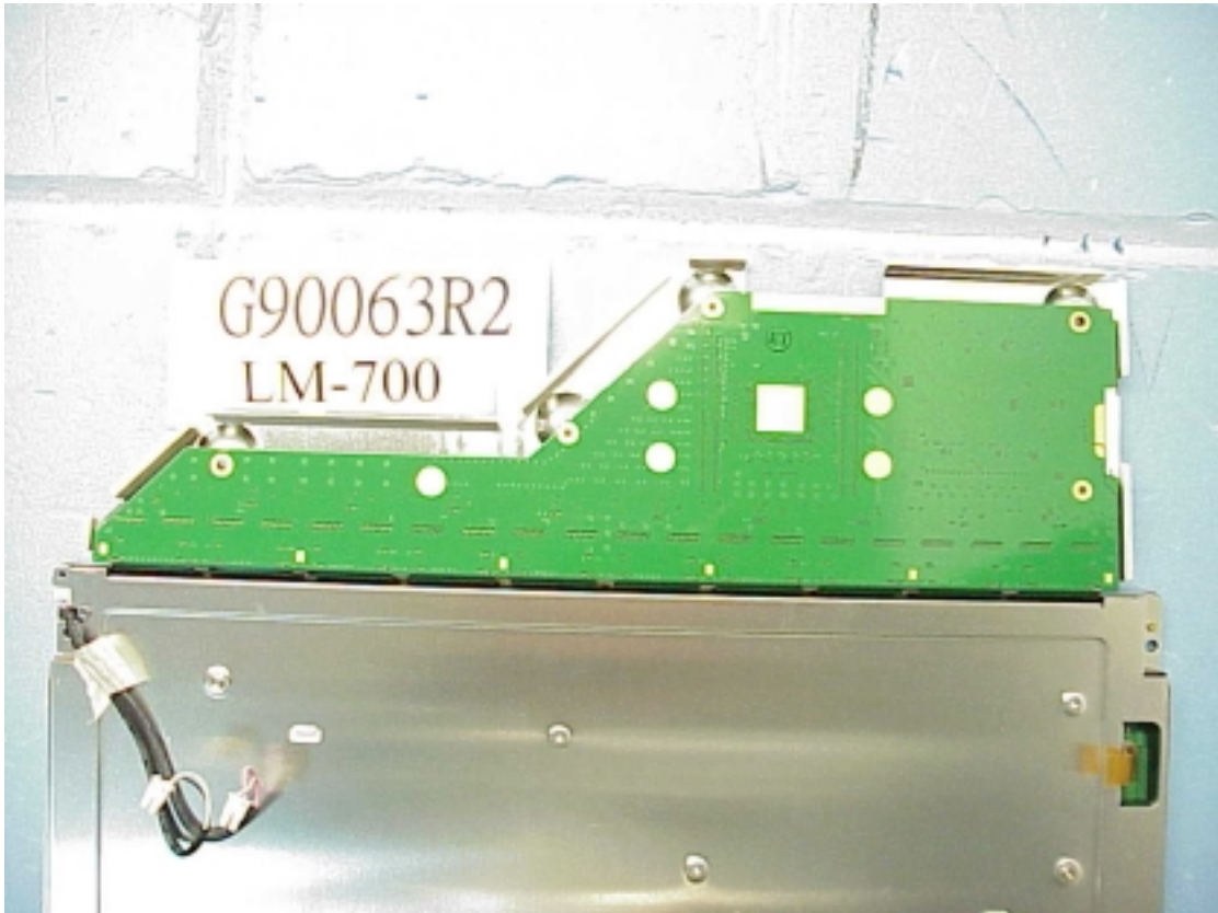
Figure 19 Control Board (Foil Side) of LCD Panel, M/N LM-700
