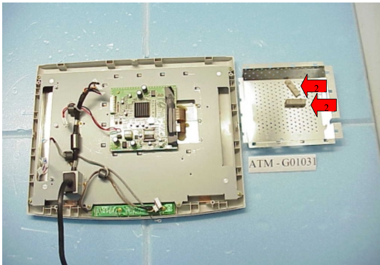
Figure 4 Internal View
