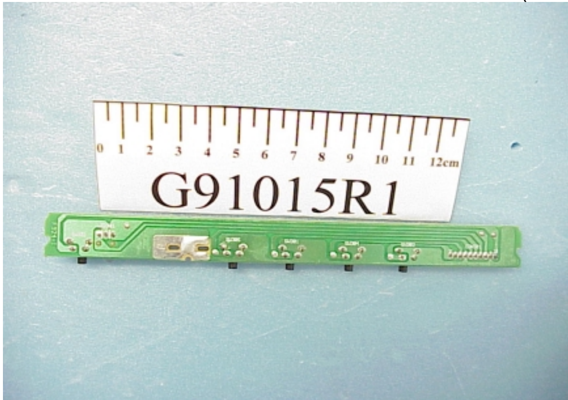
Figure 17 15" LCD Monitor OSD Control Board (Back Side)
