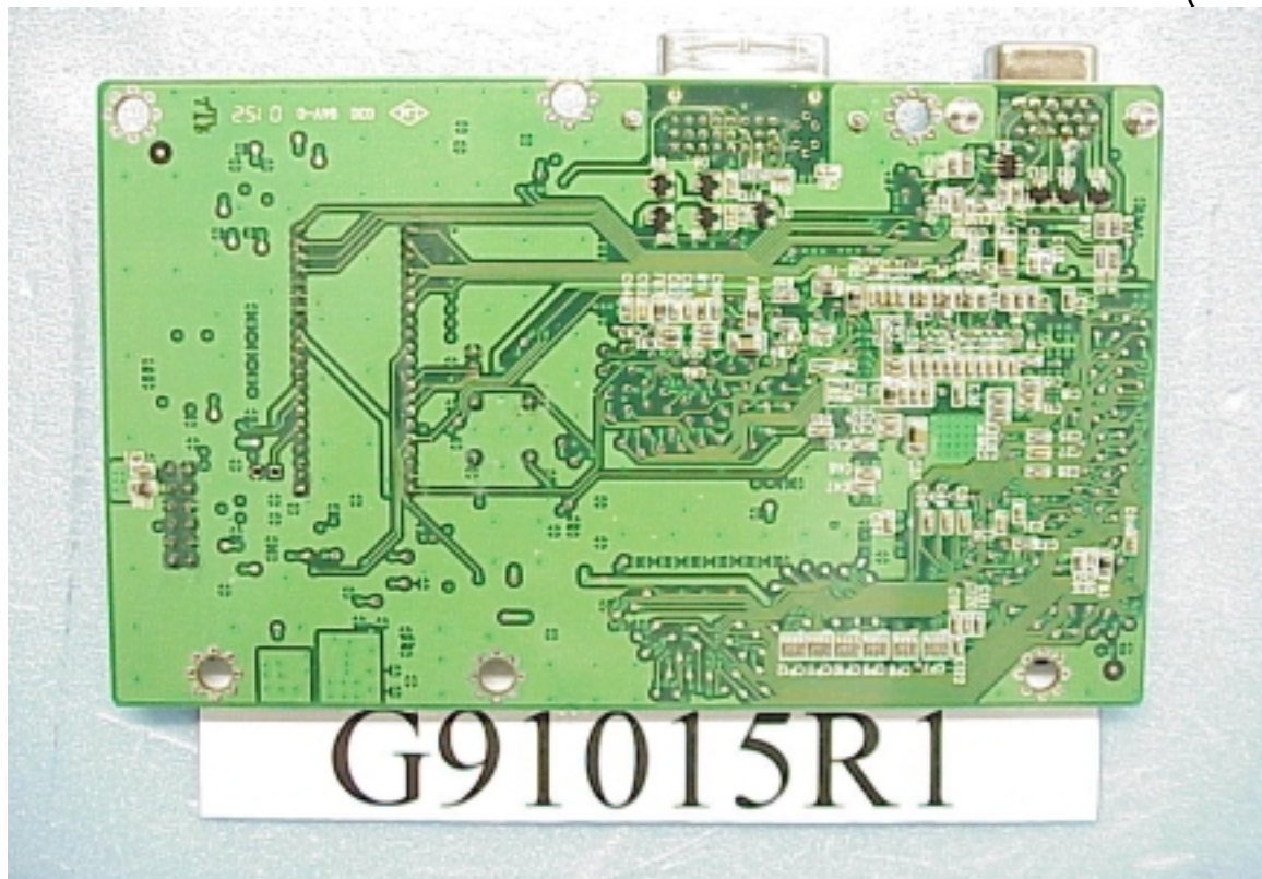
Figure 9 15" LCD Monitor Main Board (Foil Side)
