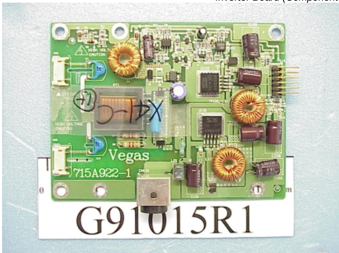
Figure 10 15" LCD Monitor Inverter Board (Component Side)
