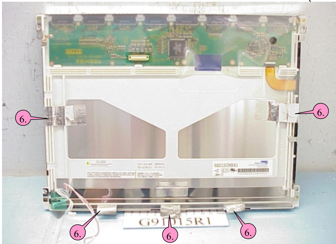
Figure 15 15" LCD Monitor LCD Panel (Rear View)
