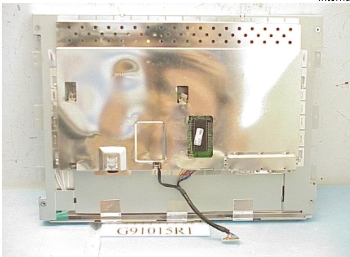
Figure 5 15" LCD Monitor Internal View
