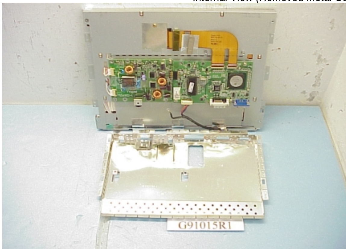
Figure 6 15" LCD Monitor Internal View (Removed Metal Cover)
