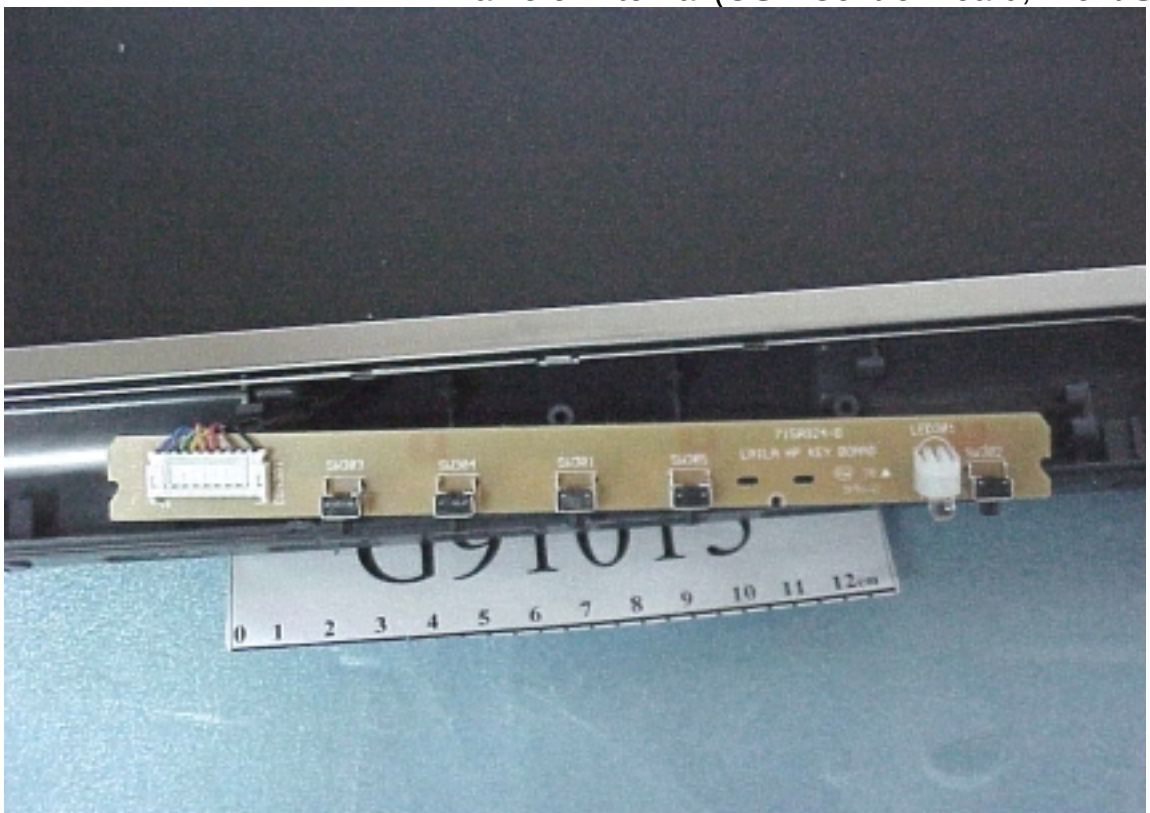
Figure 22 Frame of Internal (OSD Control Board, Front Side)
