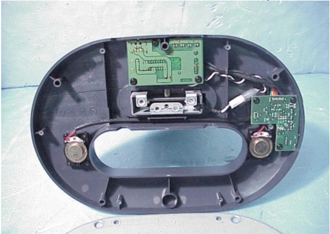
Figure 11 D5063M Base w/Audio (Frame of Internal)
