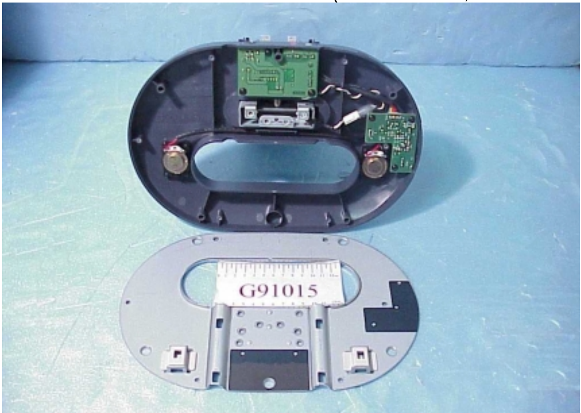
Figure 10 D5063M Base w/Audio (Removed Cover, Frame of Internal)
