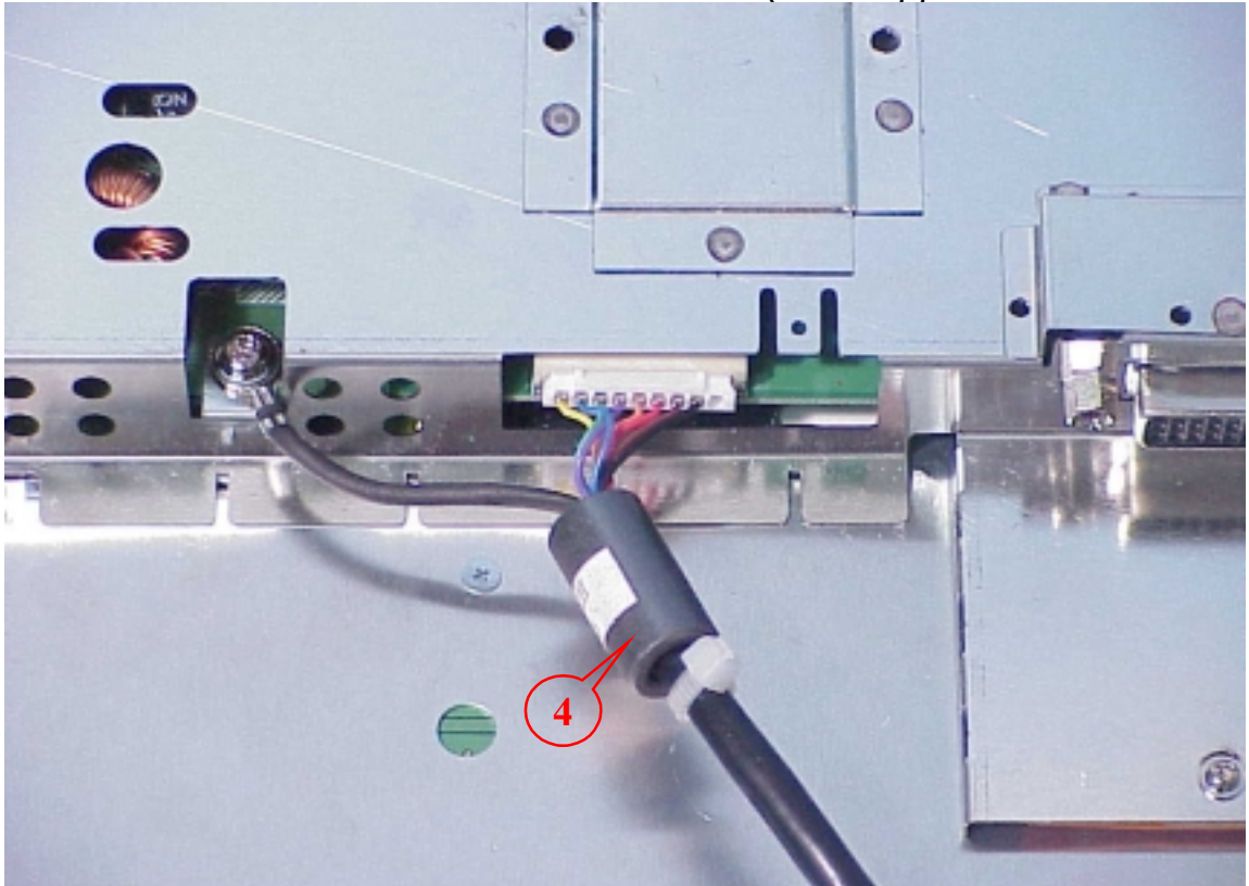
Figure 25 Frame of Internal (EMI Suppress Part-Ferrite Core)
