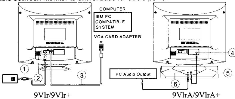
Figure 2 Connecting Cables
