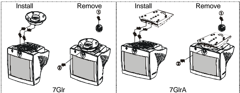
Figure 1 Installing and Removing the Swivel Base
