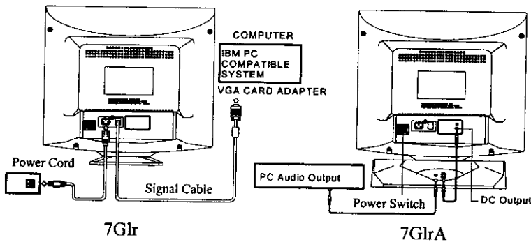
Figure 2 Connecting Cables
