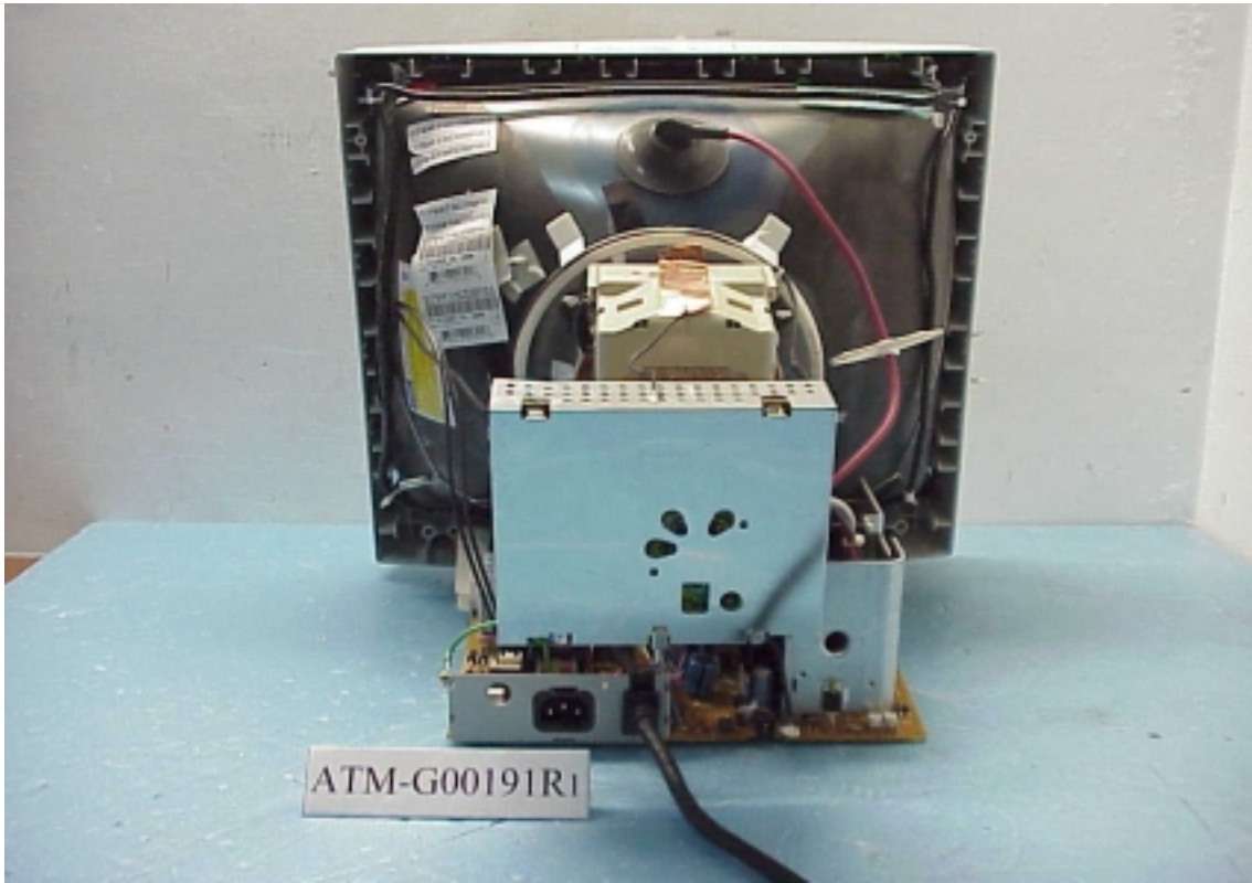
Figure 5 Internal View
