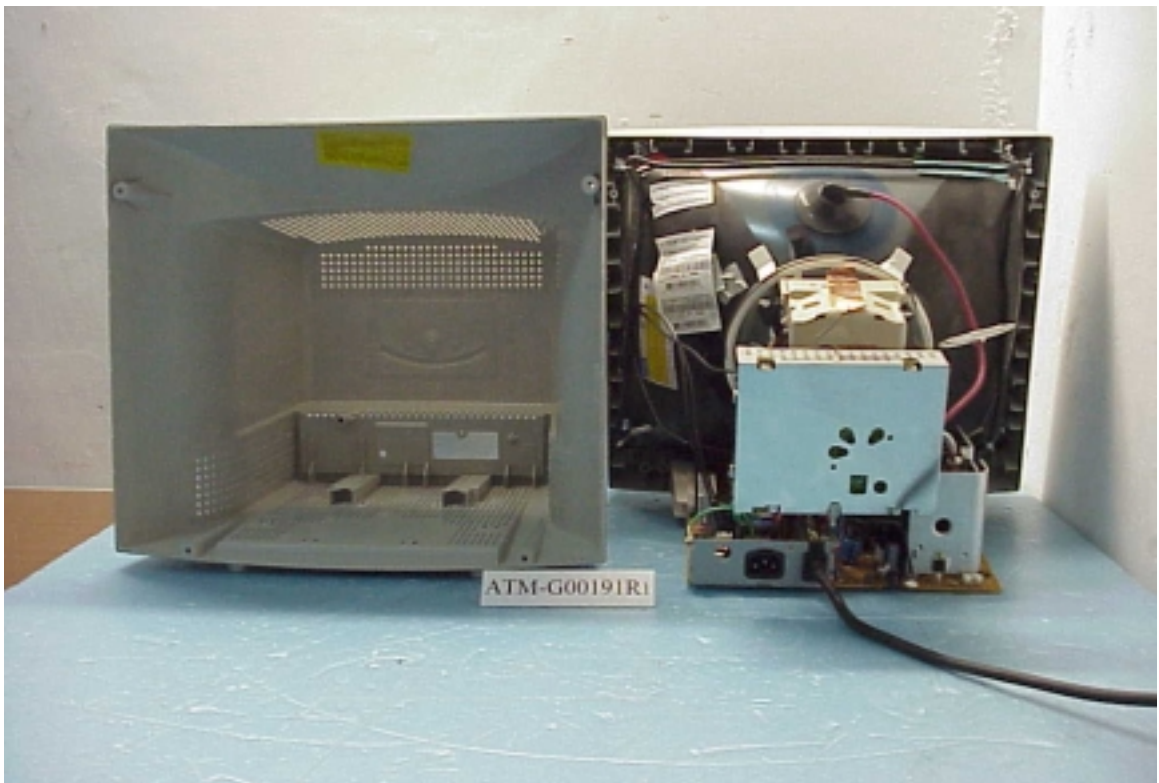
Figure 4 Internal View (Removed Back Cover)
