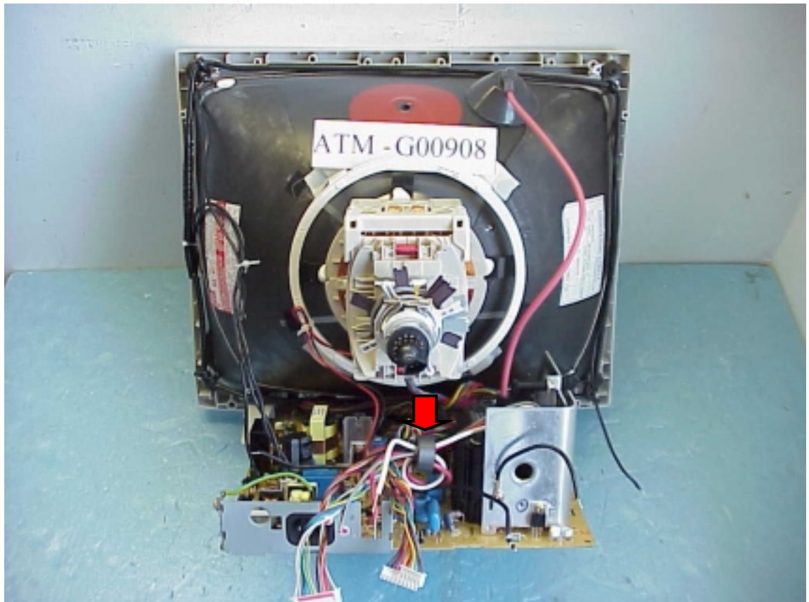
Figure 5 Internal View
