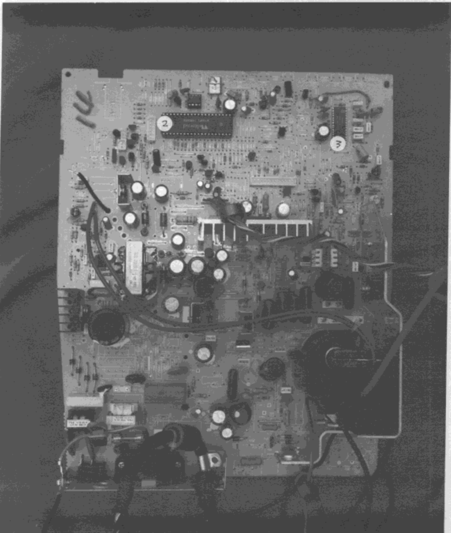
Figure 6 Main PCB Board, Component Side
