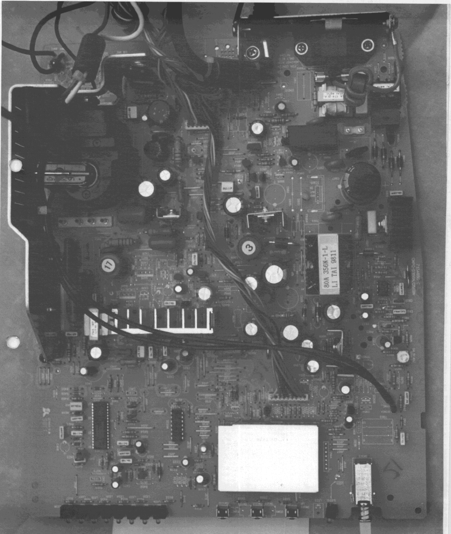
Figure 5 Main Board (Component Side)
