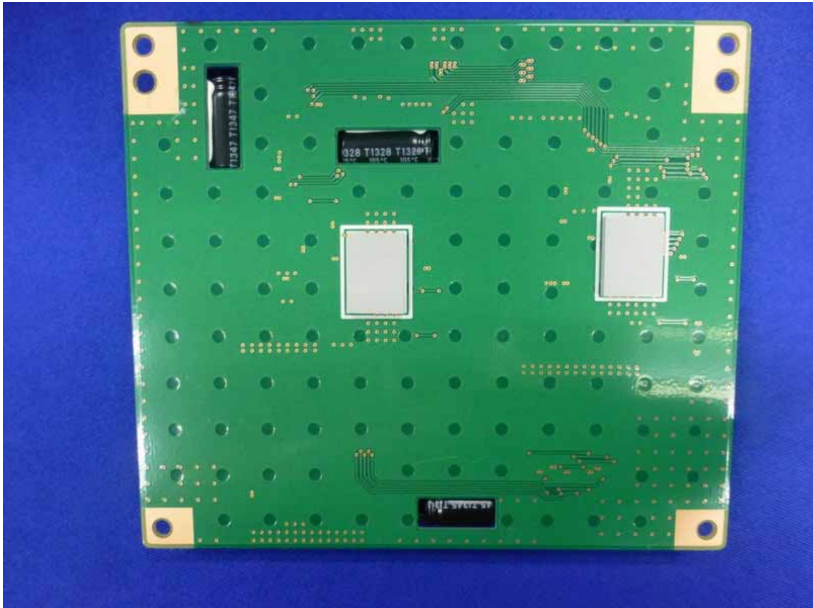
Figure 31 Backside of the PCB
