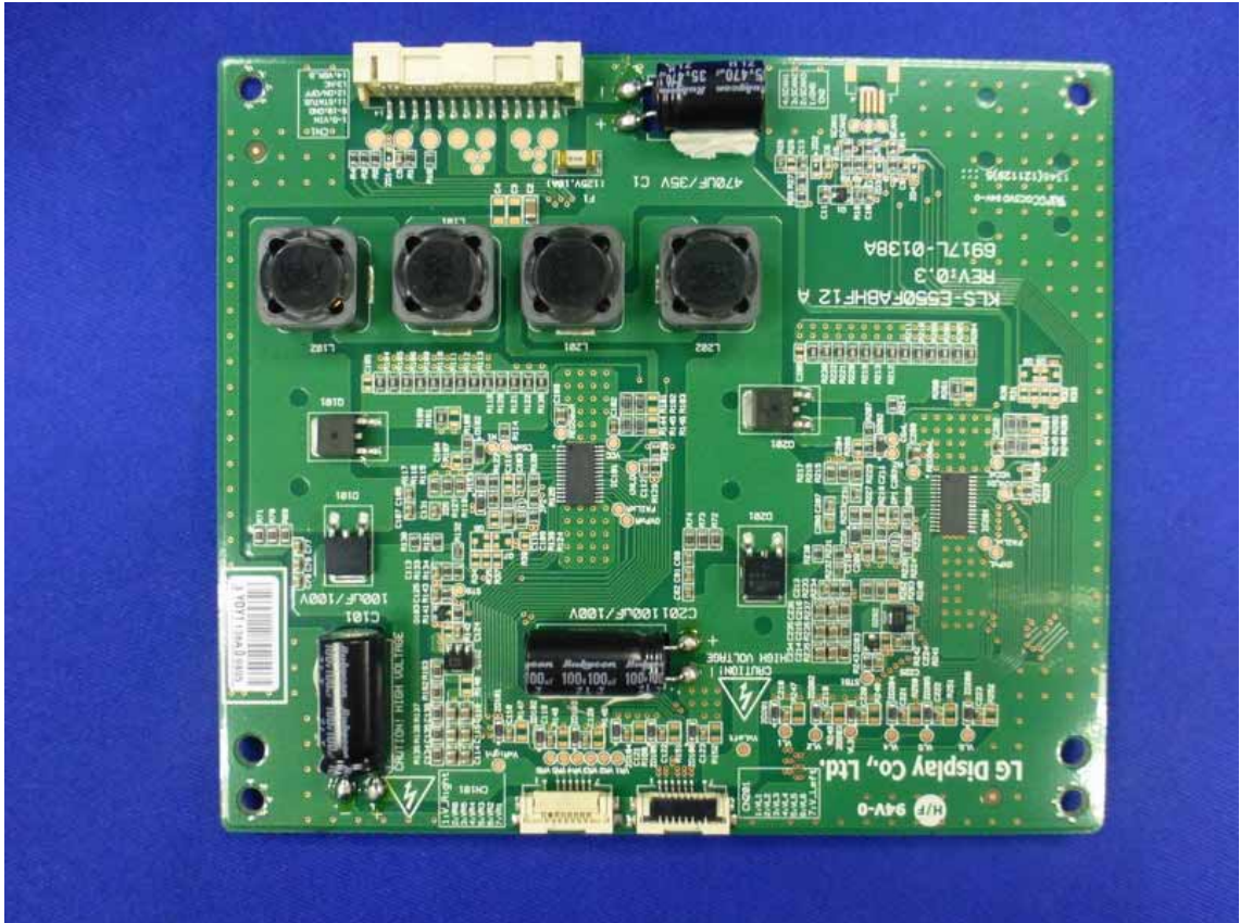
Figure 30 Frontside of the PCB
