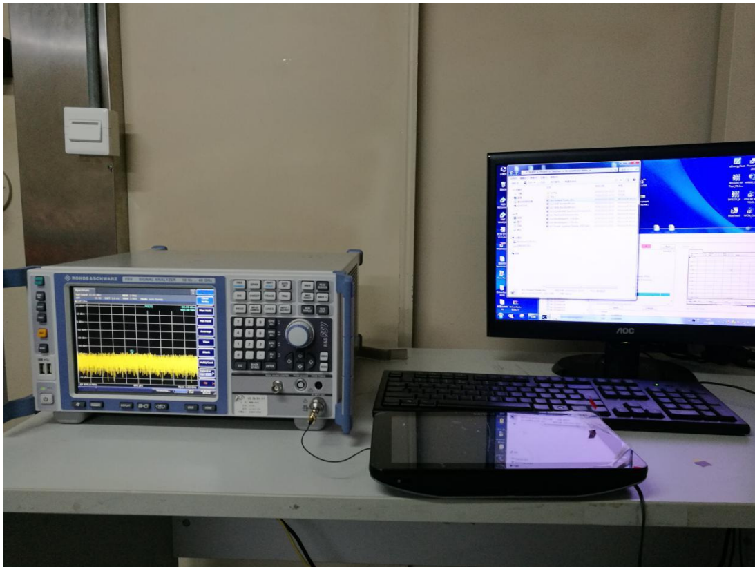
Conducted Test
