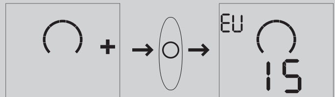
Shut-down screen
