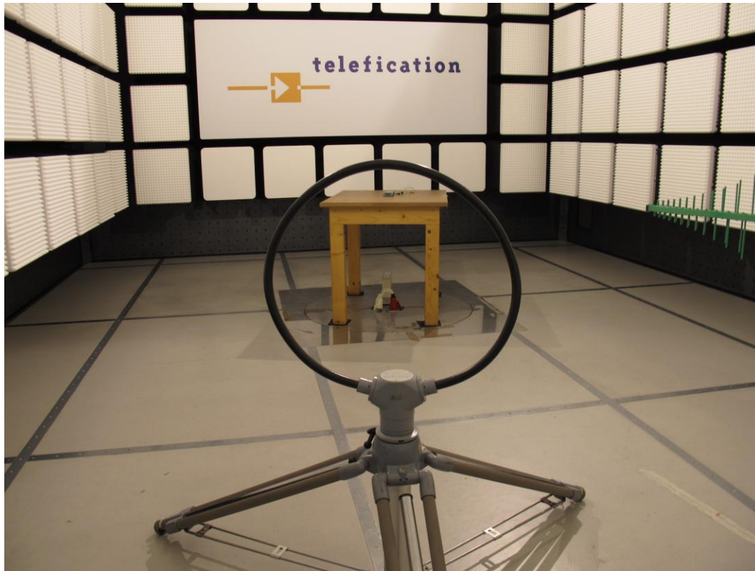
Photograph 1: Test setup radiated emissions (0.15 - 30 MHz)
