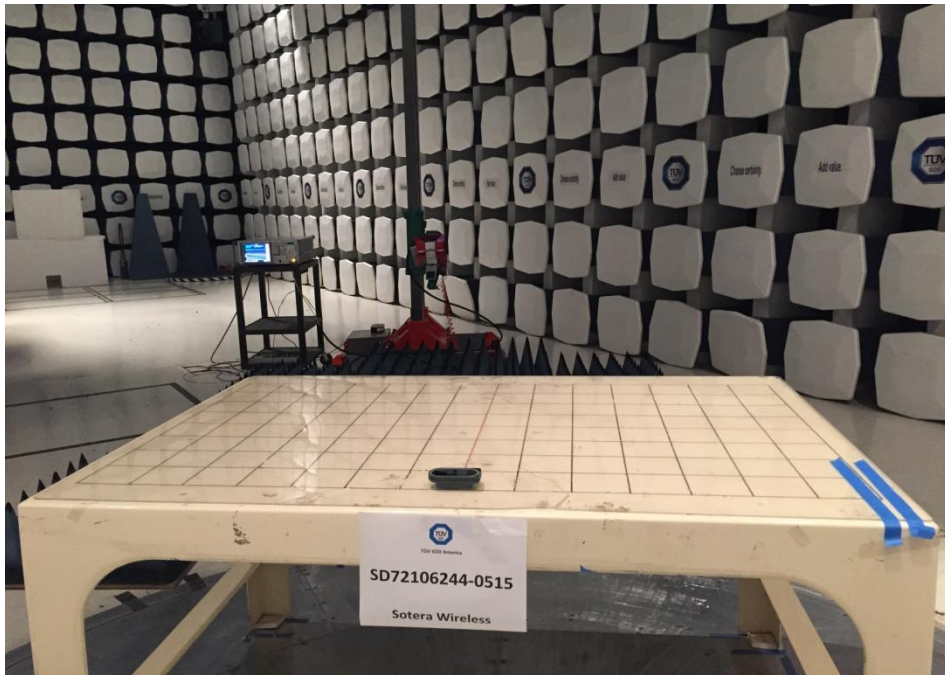
Radiated Emission Above 1GHz Front and Rear
