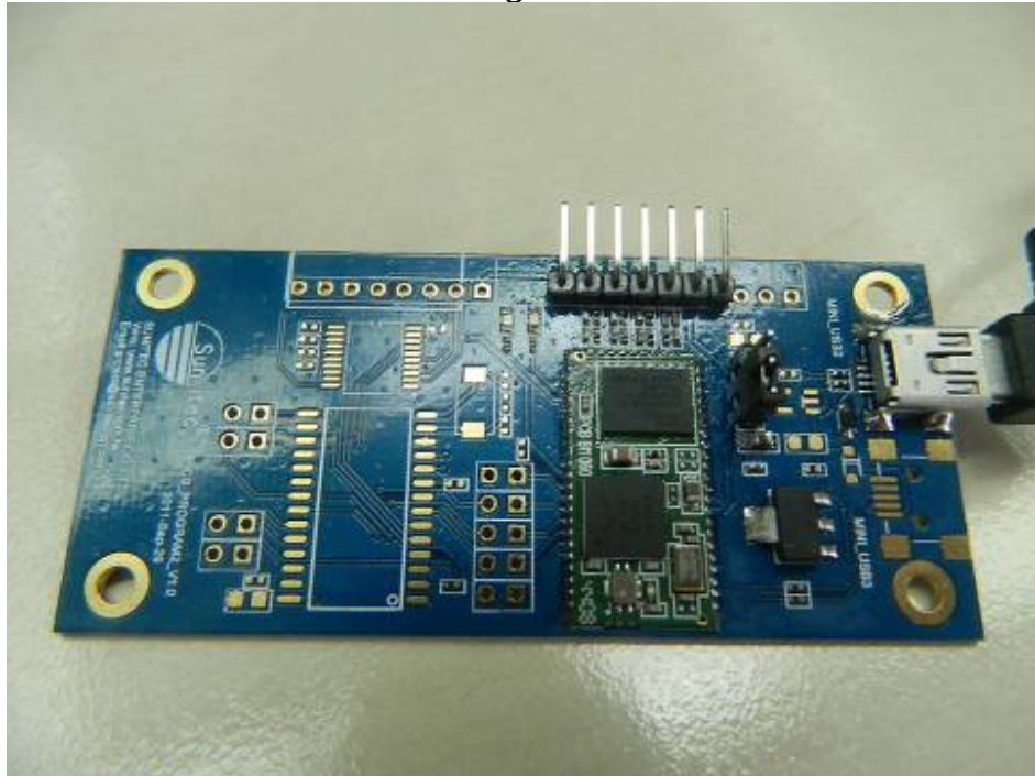
Debug Board
