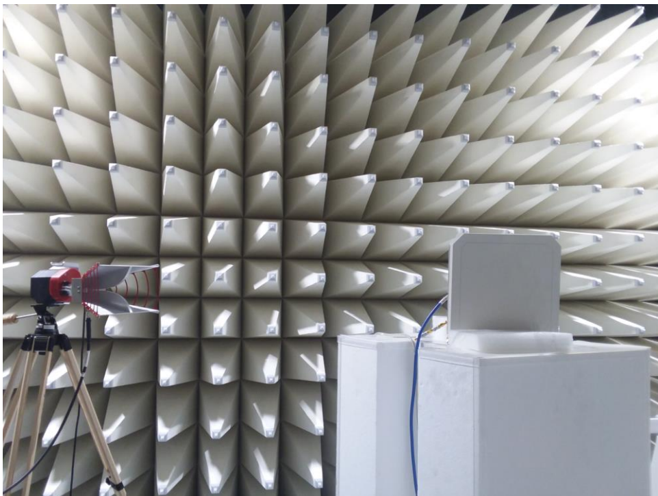
Figure B4: High Range 1-18GHz Radiated Emission test setup with horn antenna
