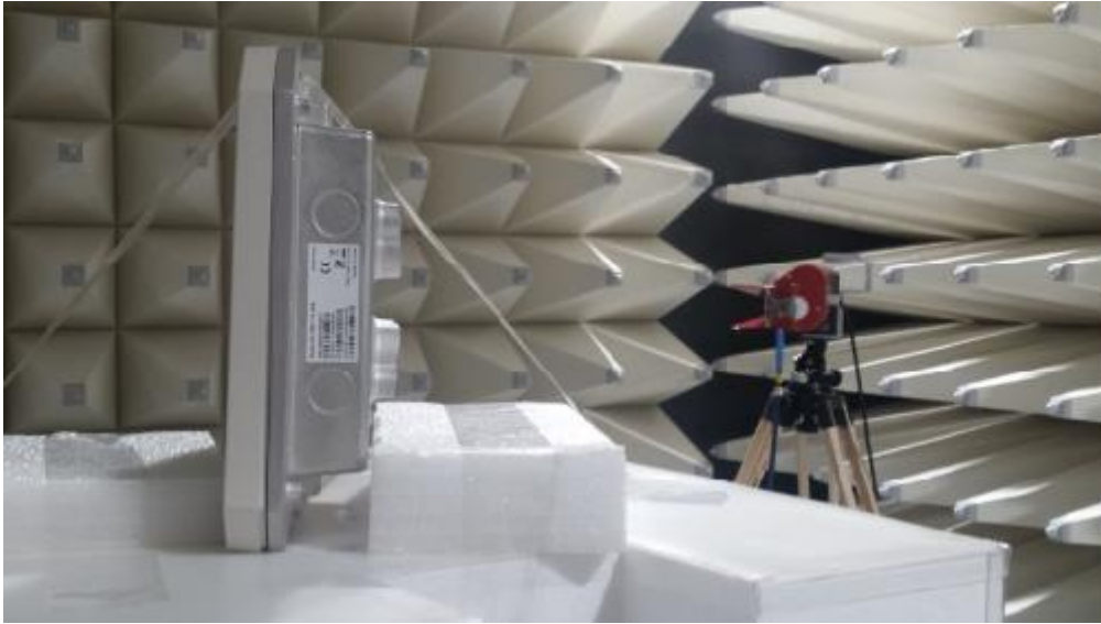
Figure B5: High Range 18-40GHz Radiated Emission test setup with horn antenna
