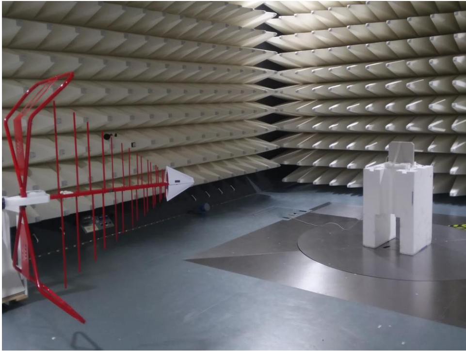
Figure B3: Low Range Radiated Emission test setup with Biconical log antenna
