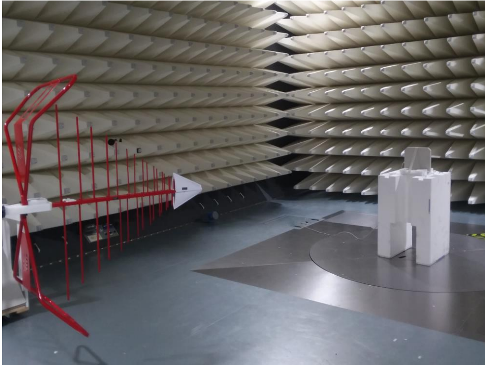
Figure B3: Low Range Radiated Emission test setup Using Biconical log antenna
