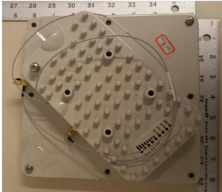
Figure B1. DUT Top View
