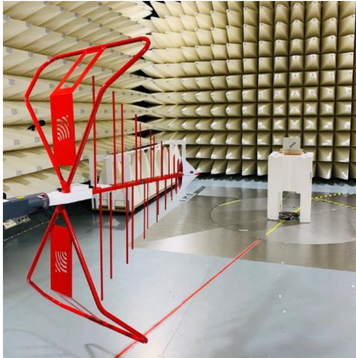
Figure B3. Radiated Setup 1
