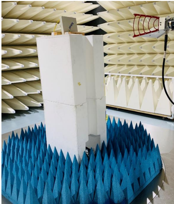
Figure B4. Radiated Setup 2
