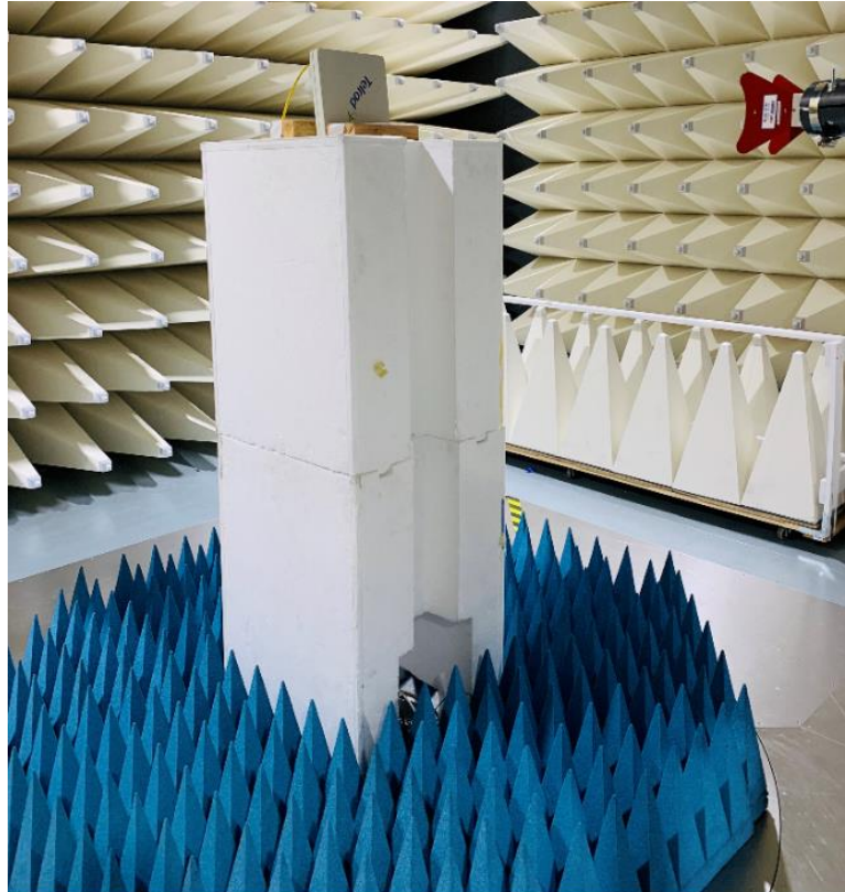
Figure B5. Radiated Setup 3
