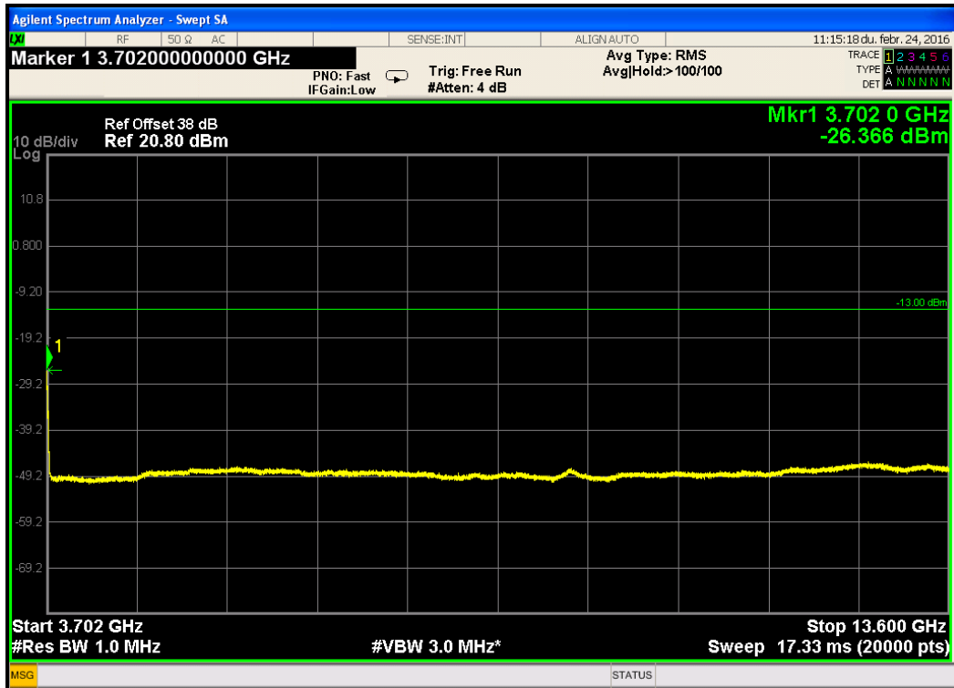
Figure 269. — 15MHz CBW - 3702.0MHz -13.6GHz band, top frequency, 64QAM
