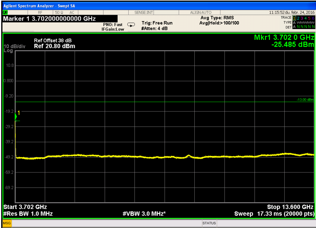
Figure 274.— 15MHz CBW - 3702.0MHz -13.6GHz band, top frequency, 16QAM
