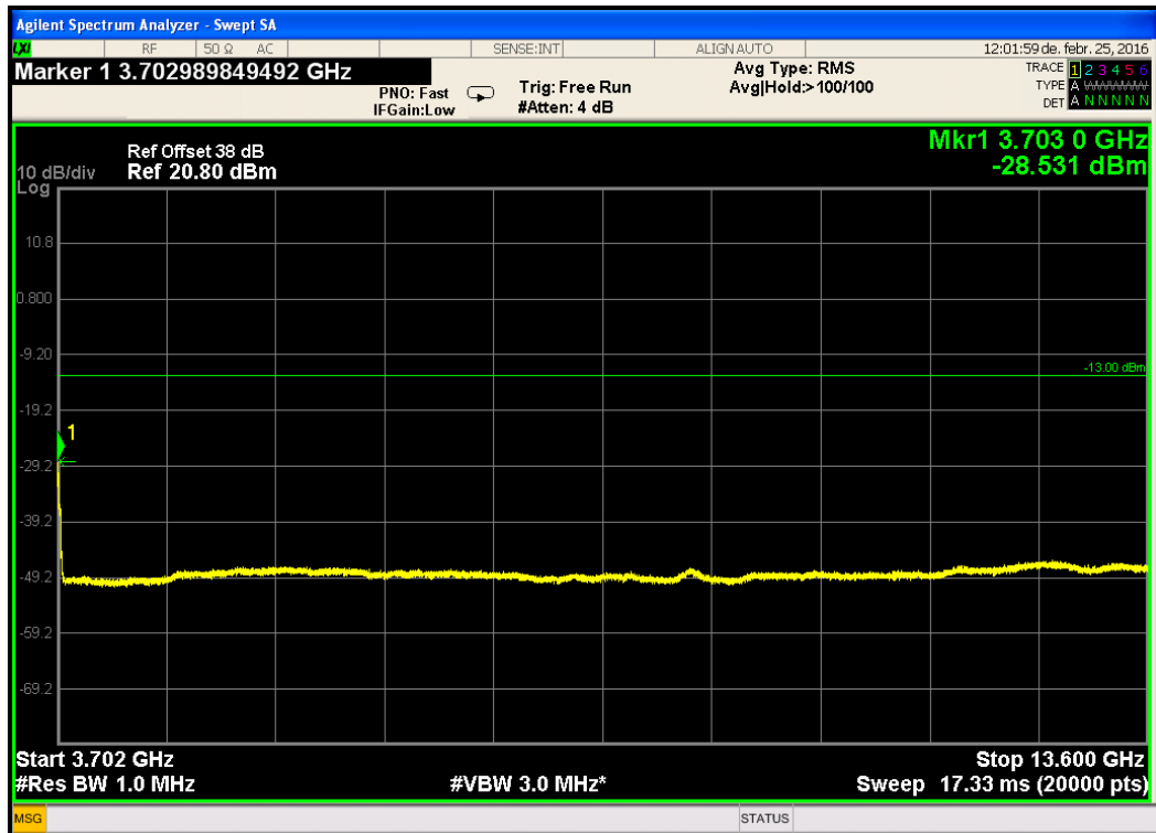
Figure 309.— 20MHz CBW - 3702.0MHz -13.6GHz band, top frequency, QPSK
