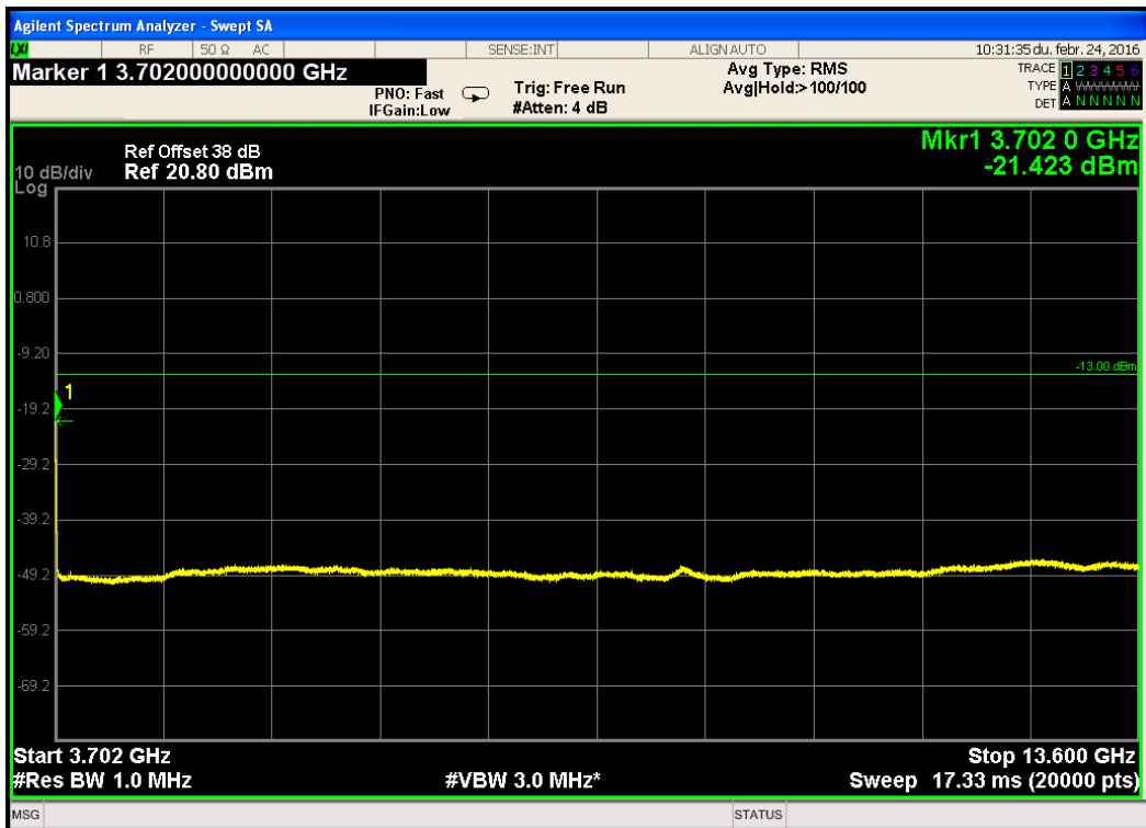
Figure 249.— 10MHz CBW - 3702.0MHz -13.6GHz band, top frequency, QPSK
