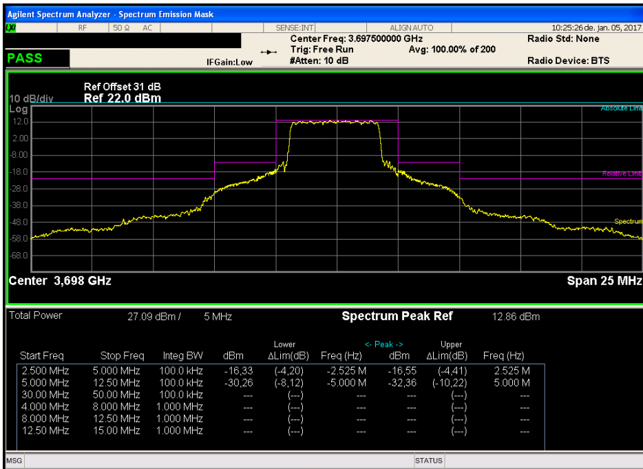
Figure 162. —5MHz CBW – High Frequency, 16QAM
