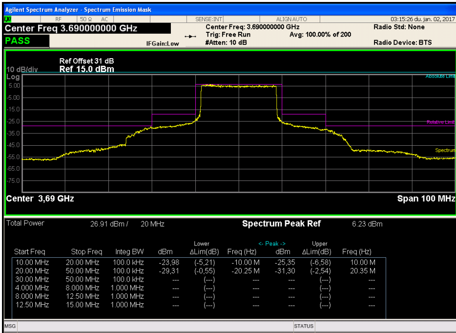
Figure 188. —20MHz CBW – High Frequency, 64QAM
