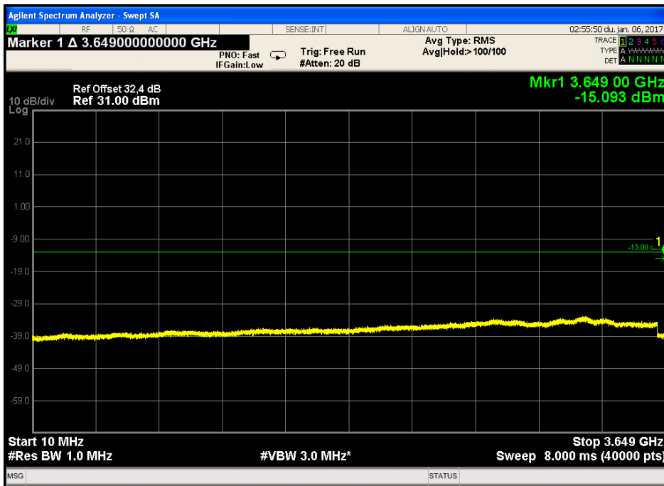
Figure 202. —5MHz CBW - 10.0MHz-3649.0MHz band, bottom frequency, QPSK
