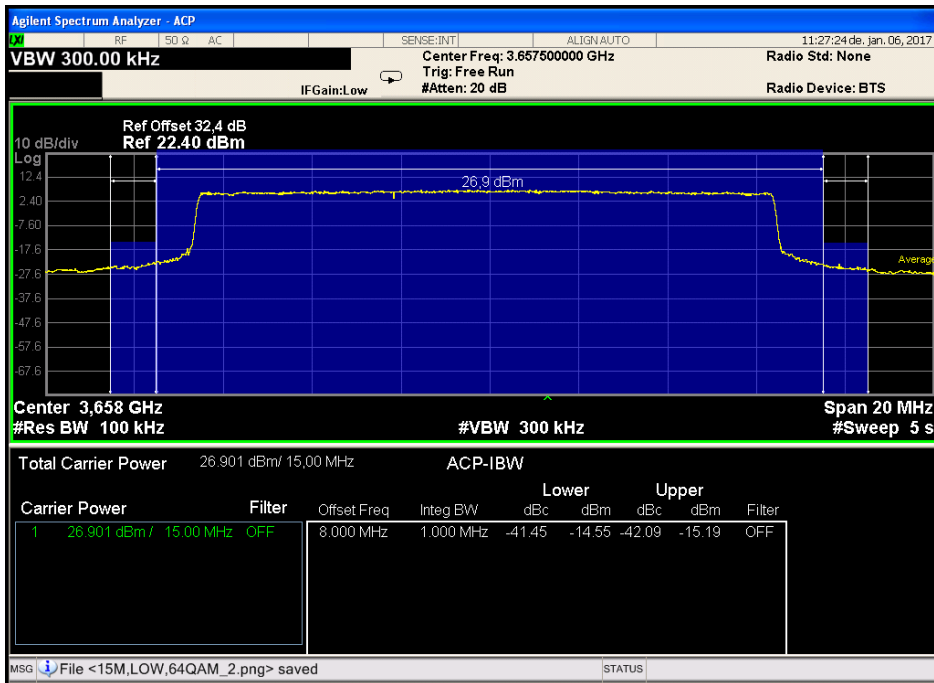
Figure 253.— 15MHz CBW - 3649.0MHz-3650.0MHz band, bottom frequency, 64QAM
