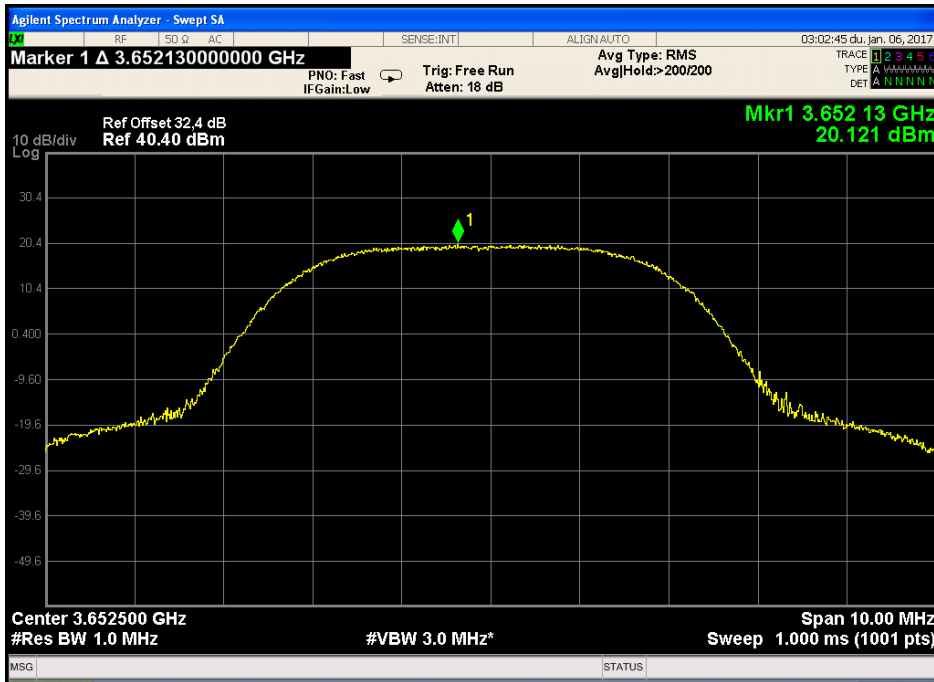
Figure 116. — 3652.5 MHz QPSK - 5MHz CBW, Low Population
