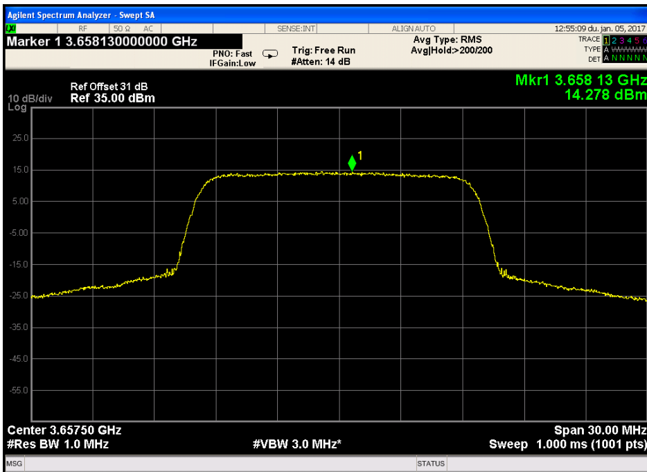
Figure 99. — 3657.5MHz 16QAM - 15MHz CBW, High Population
