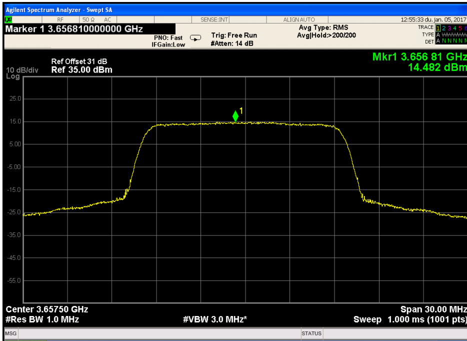
Figure 98. — 3657.5MHz QPSK - 15MHz CBW, High Population
