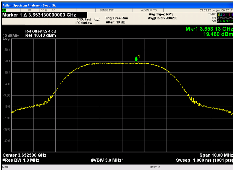
Figure 117. — 3652.5 MHz 16QAM - 5MHz CBW, Low Population
