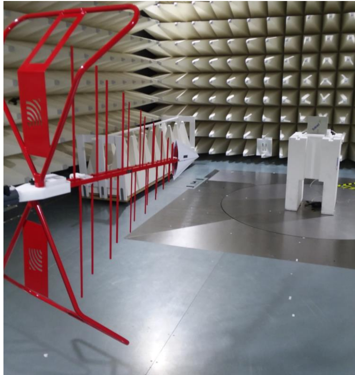
Figure B3: Low Range Radiated Emission test setup Using Biconical log antenna
