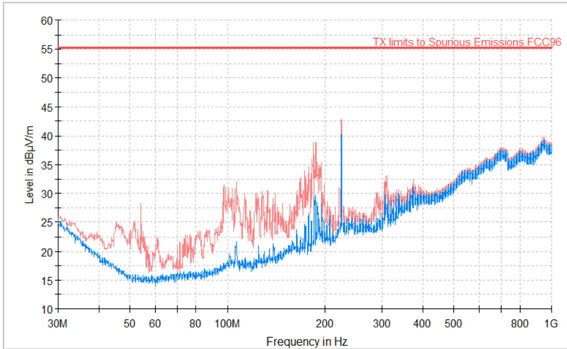
RF_FCC_Part96_E Field_30MHz_1GHz
