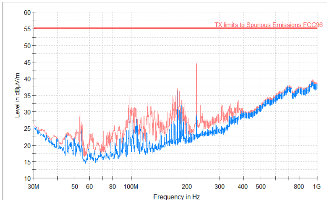
RF_FCC_Part96_E Field_30MHz_1GHz
