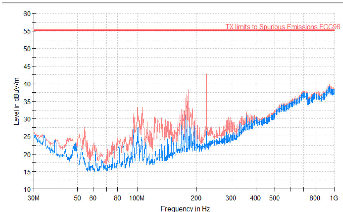
RF_FCC_Part96_E Field_30MHz_1GHz
