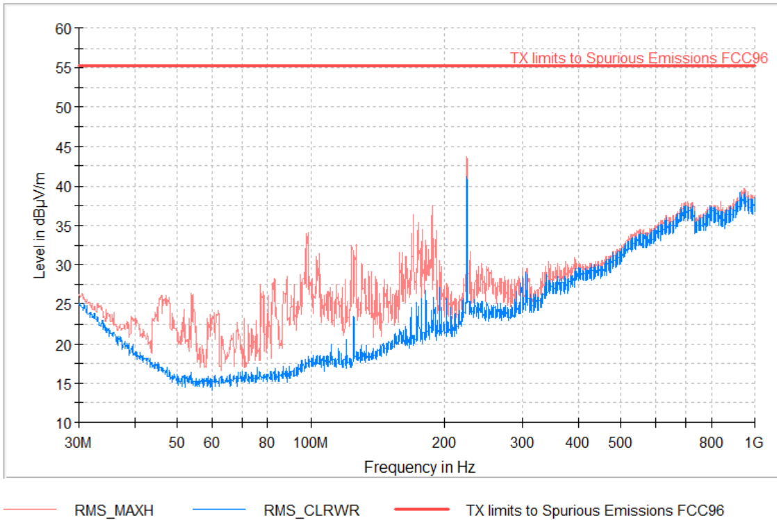
RF_FCC_Part96_E Field_30MHz_1GHz
