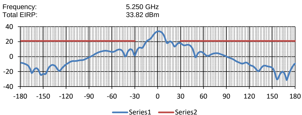
Plot 7.15.8 Antenna pattern test results, Antenna #4
