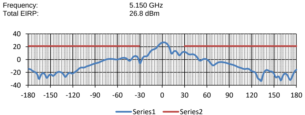
Plot 7.15.4 Antenna pattern test results, Antenna #4
