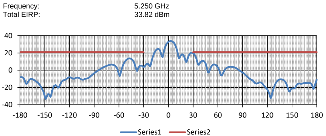
Plot 7.15.5 Antenna pattern test results, Antenna #1
