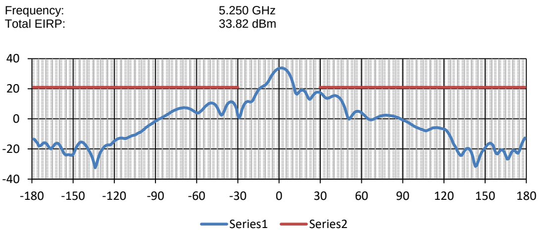
Plot 7.15.6 Antenna pattern test results, Antenna #2
