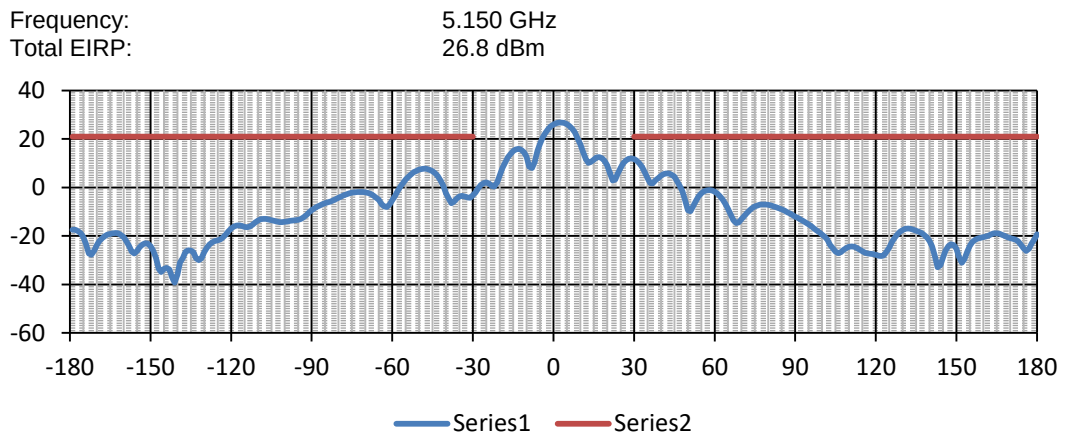
Plot 7.15.1 Antenna pattern test results, Antenna #1
