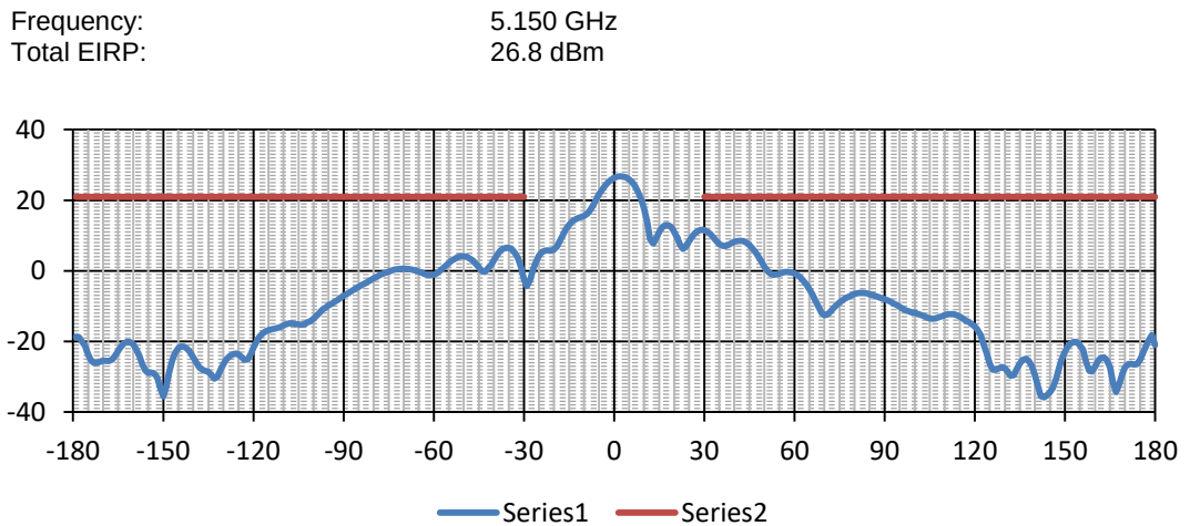
Plot 7.15.2 Antenna pattern test results, Antenna #2
