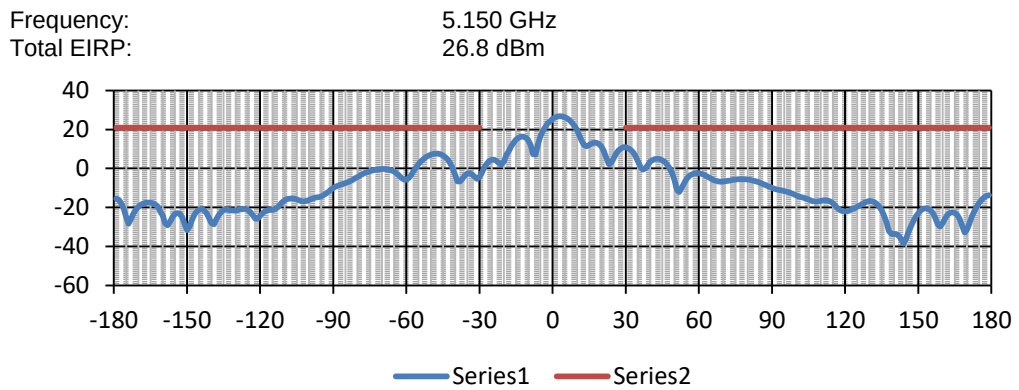
Plot 7.15.3 Antenna pattern test results, Antenna #3
