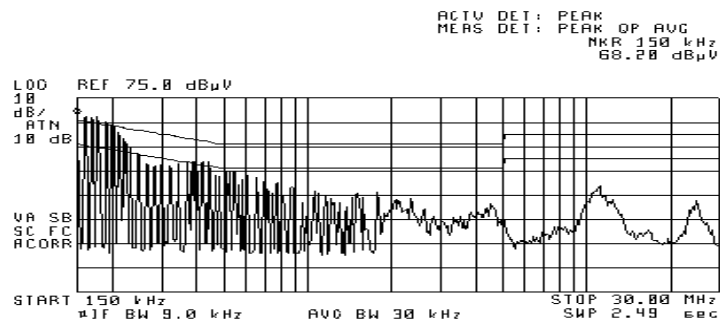
Plot 7.14.2 Conducted emission measurements
