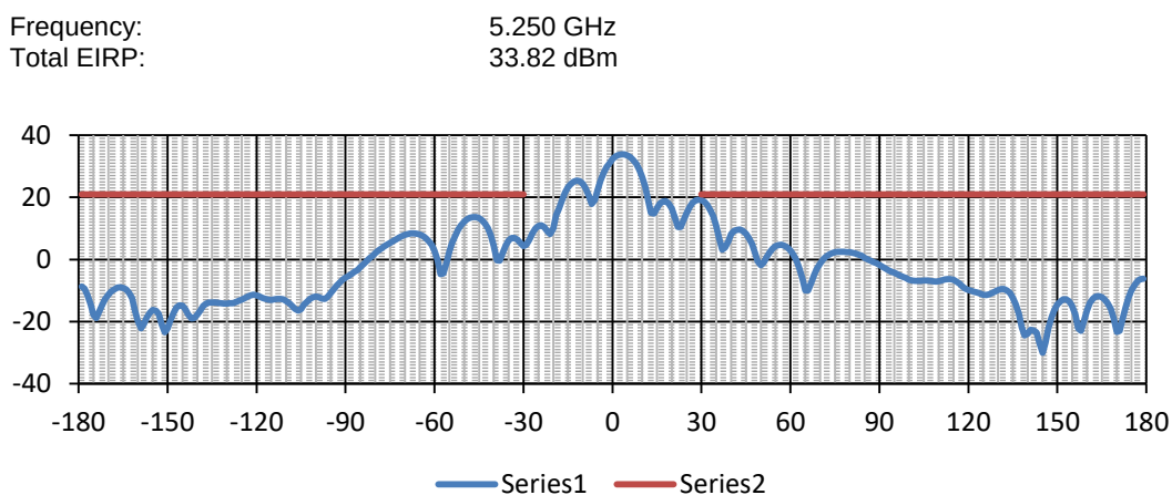
Plot 7.15.7 Antenna pattern test results, Antenna #3
