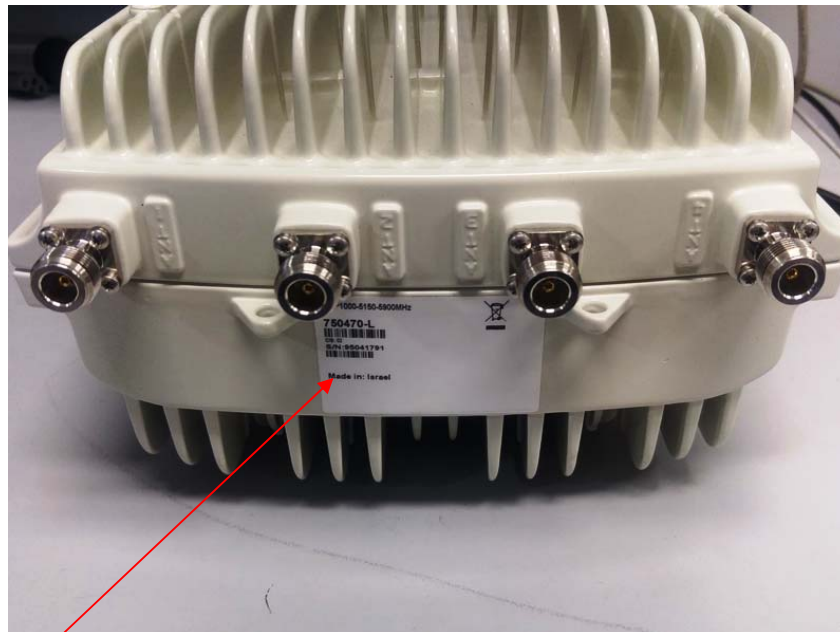
Label with FCC ID:ARA-COMPACT5X and IC:899A-COMPACT5X location.
