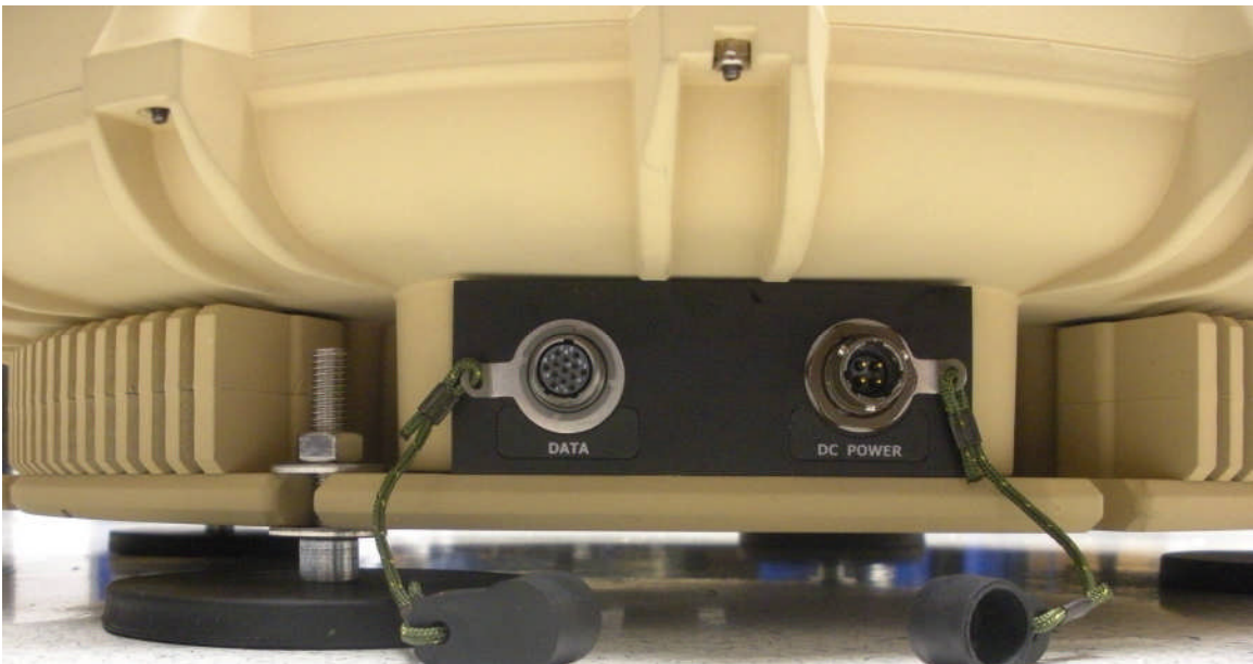
Land Mobile BGAN Terminal, RF-7800B-VU104 Side view – Connectors Uncovered
