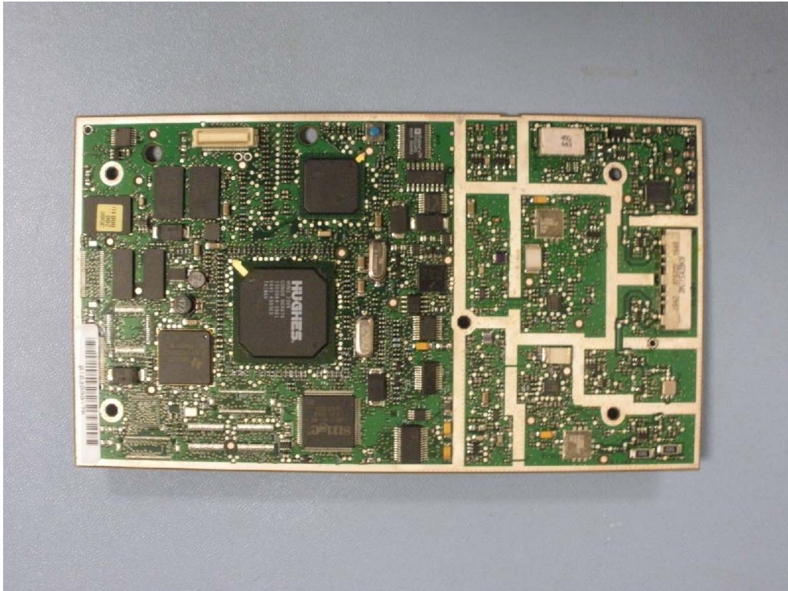
Land Mobile BGAN Terminal, RF-7800B-VU104 Core Module Without Shield - Topside
