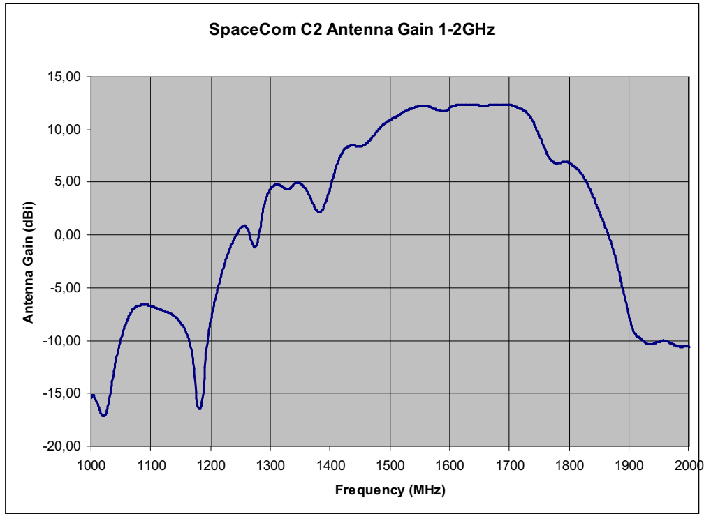
Figure 5-2: C2 Antenna gain 1-2GHz.
