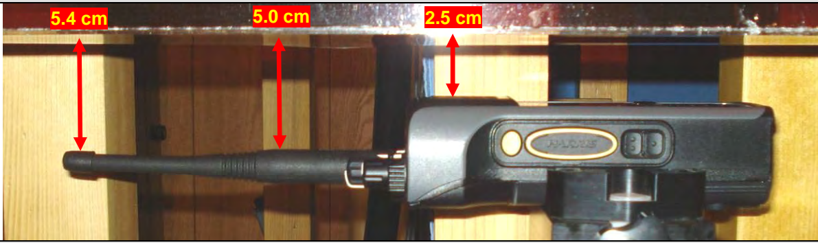
Face-held with Battery b and Antenna #1
