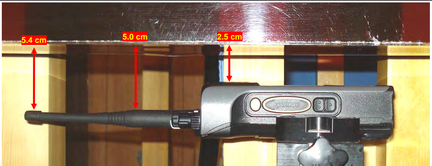
Face-held with Battery c and Antenna #1
