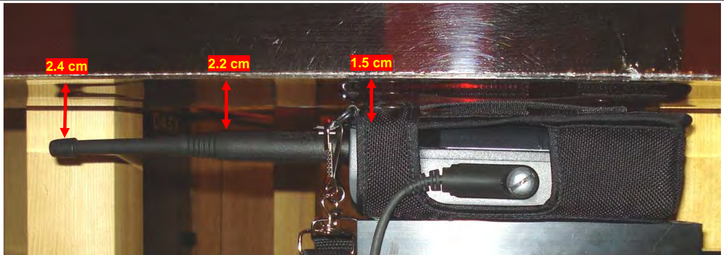
Body-worn Accessory B4, Audio Accessory A1, and Antenna #1
