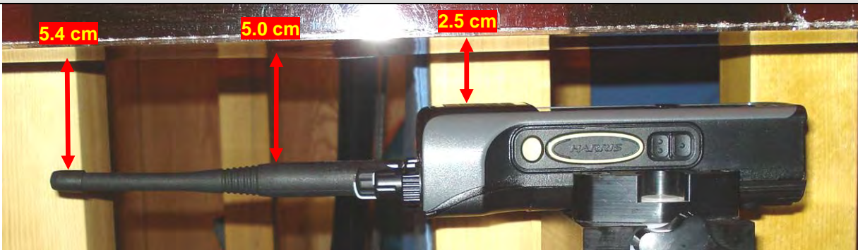
Face-held with Battery e and Antenna #1
