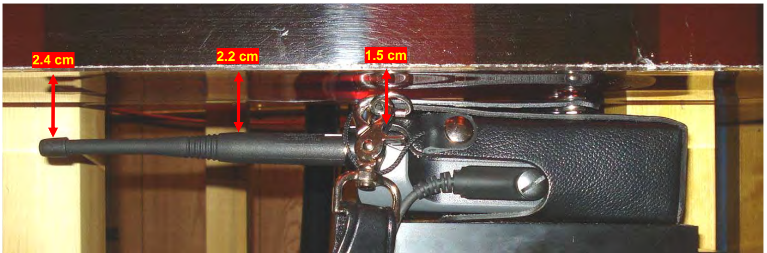
Body-worn Accessory B7, Audio Accessory A1, and Antenna #1
