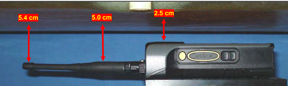
Face-held with Battery e and Antenna #1
