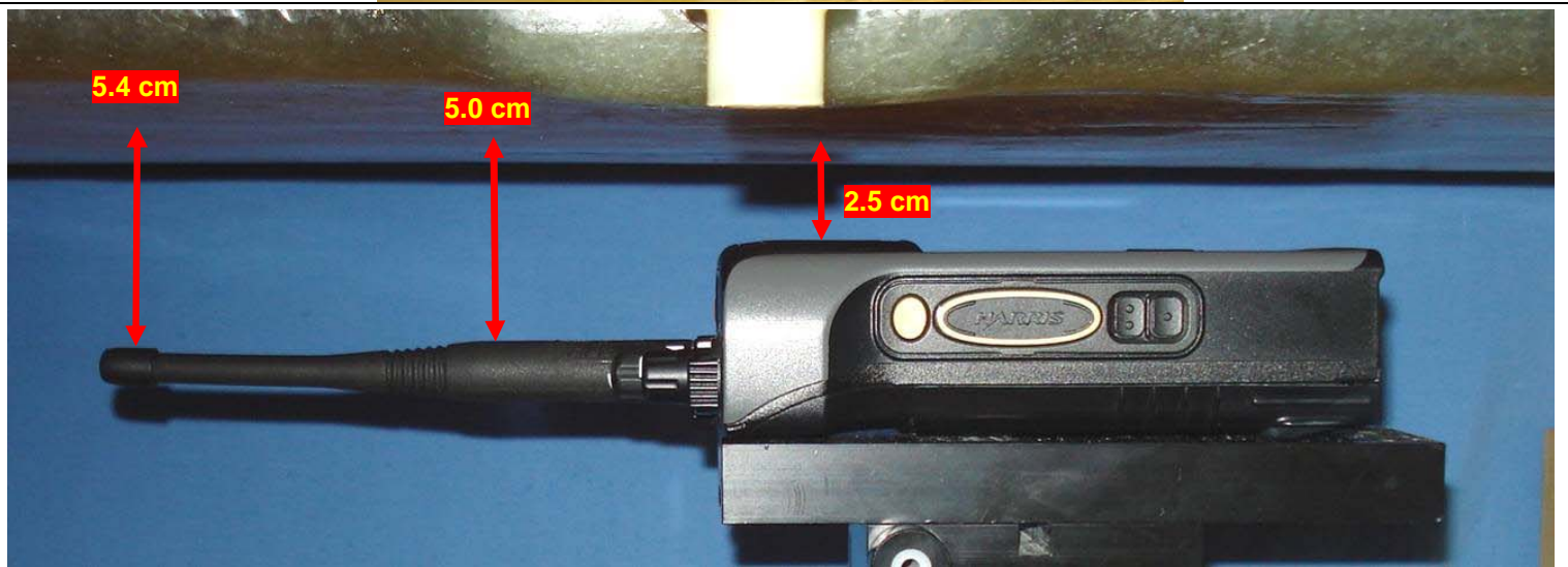
Face-held with Battery c and Antenna #1
