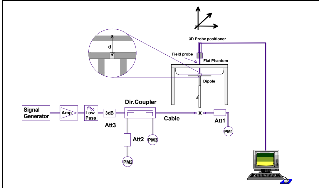
System Performance Check Measurement Setup Diagram (IEEE 1528-2003) 450 MHz SPEAG Validation Dipole Setup
