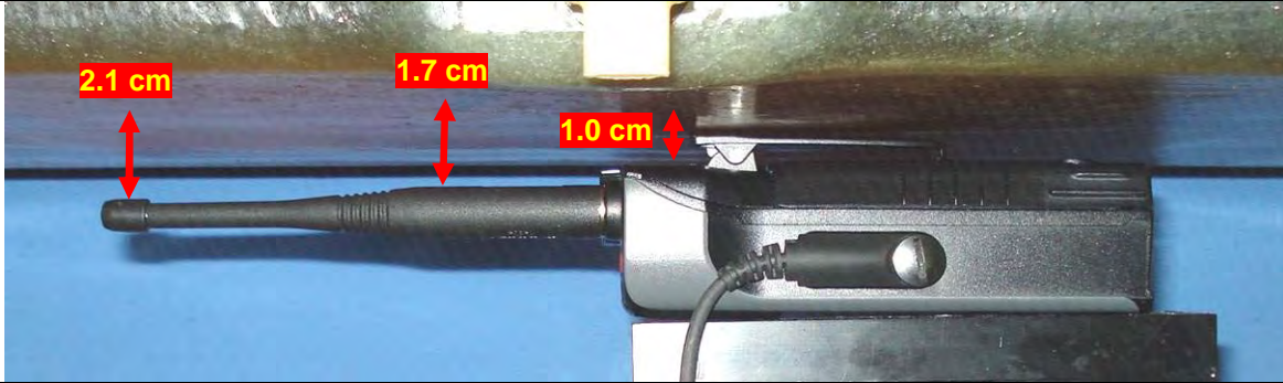
Body-worn Accessory B1, Battery a, Audio Accessory A1, and Antenna #1
