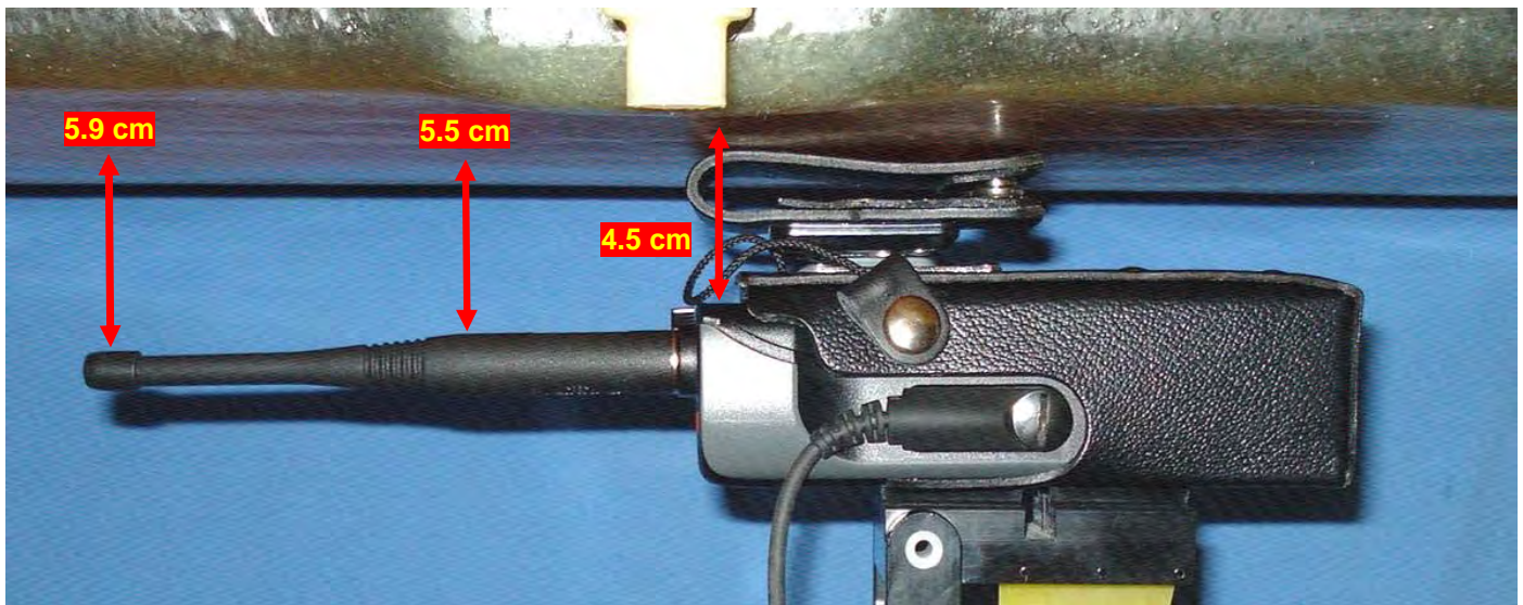
Body-worn Accessory B10, Audio Accessory A1, and Antenna #1
