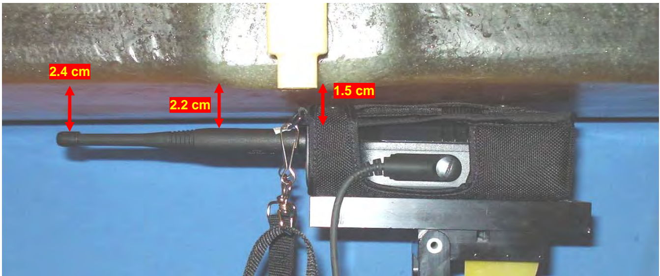
Body-worn Accessory B4, Audio Accessory A1, and Antenna #1
