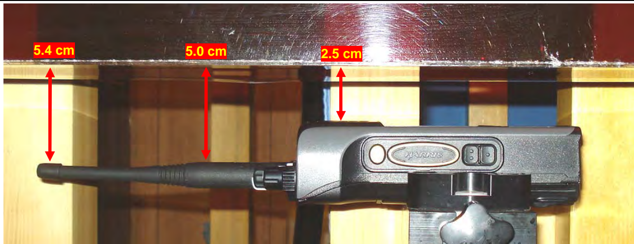
Face-held with Battery c and Antenna #1
