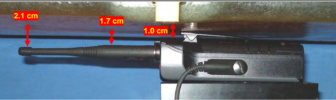
Body-worn Accessory B1, Battery e, Audio Accessory A1, and Antenna #1
