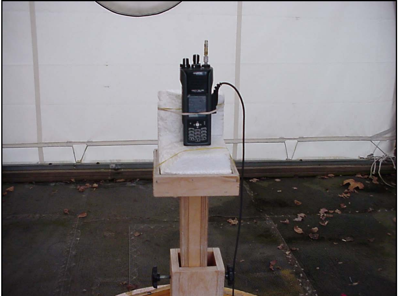
Photograph 2: Radiated Emissions – Front View
