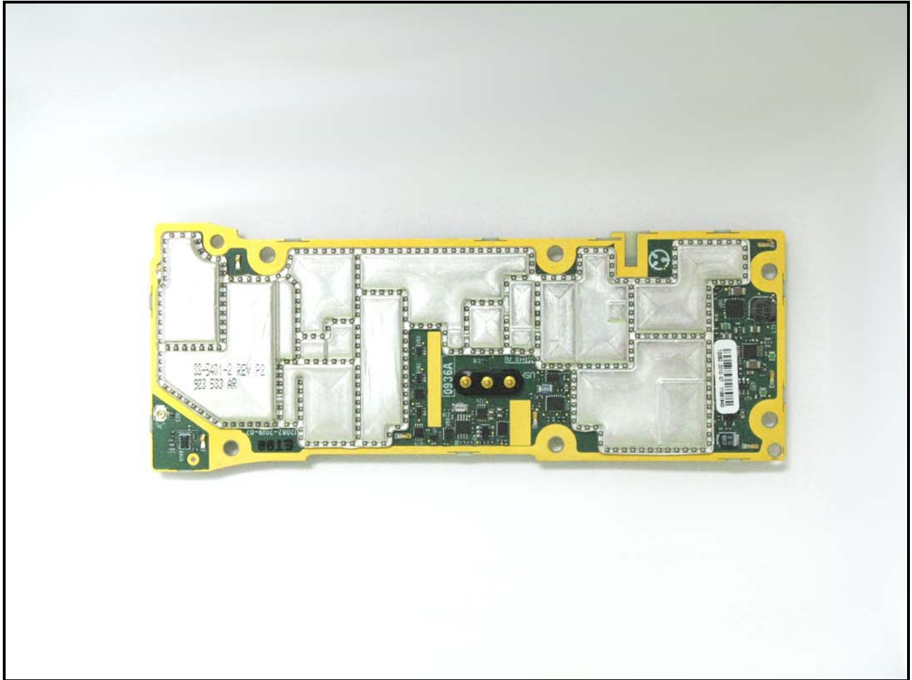
Photograph 12: RF PWB Side 2 Shielded
