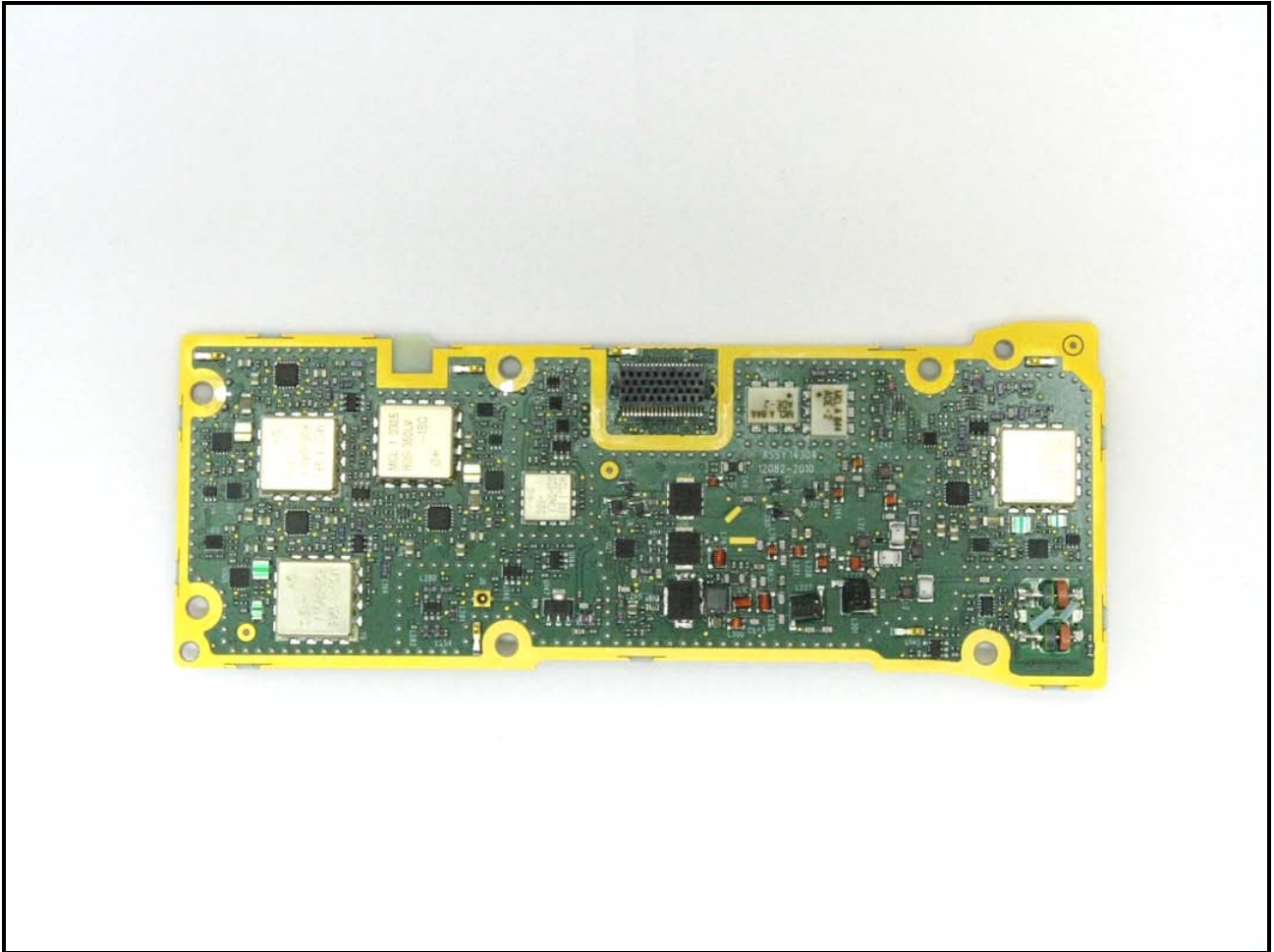
Photograph 11: RF PWB Side 1 Unshielded
