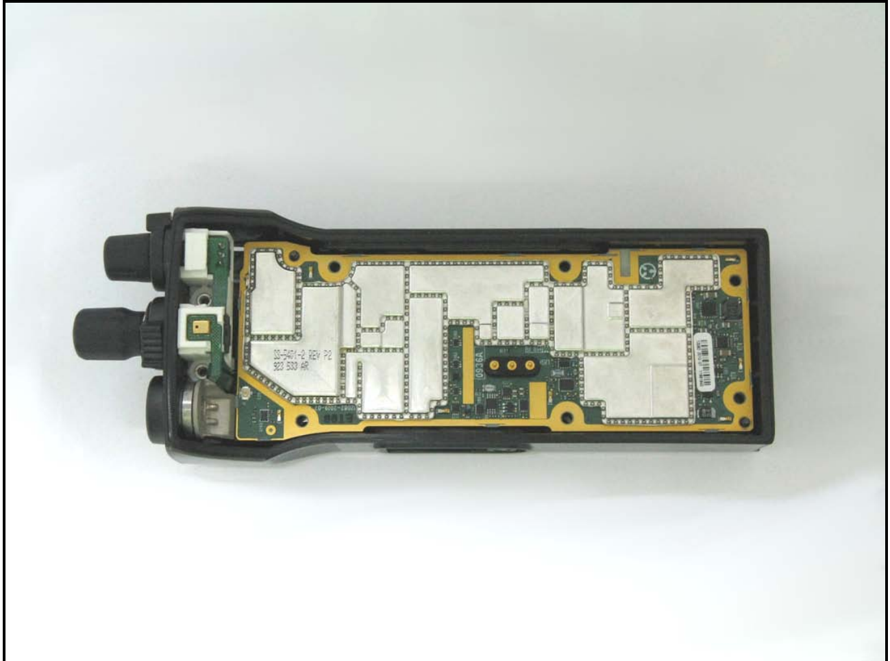
Photograph 9: RF PWB in Chassis
