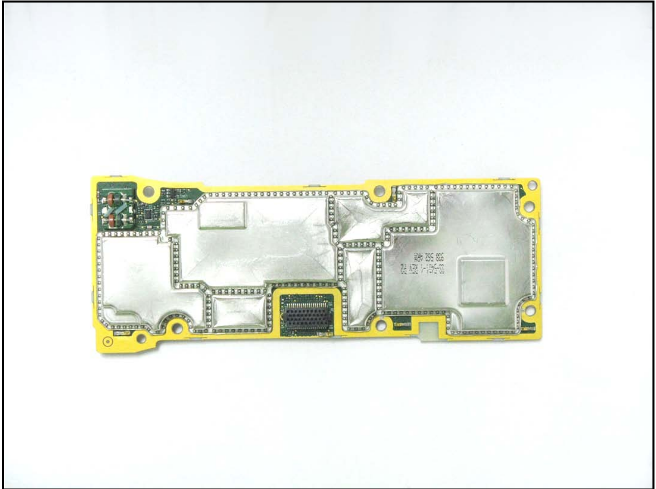
Photograph 10: RF PWB Side 1 Shielded
