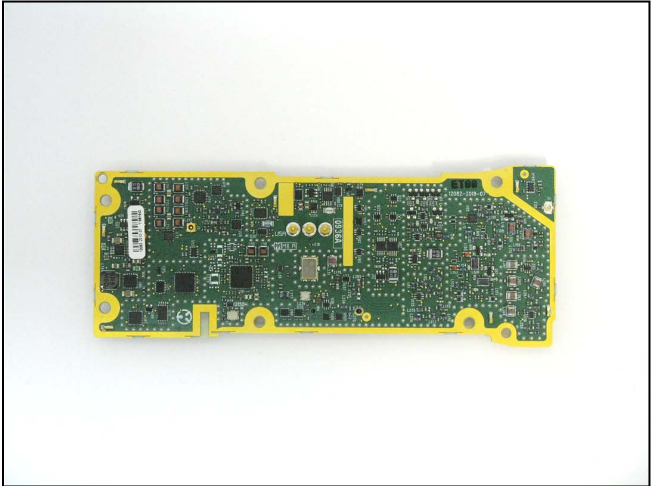
Photograph 13: RF PWB Side 2 Unshielded
