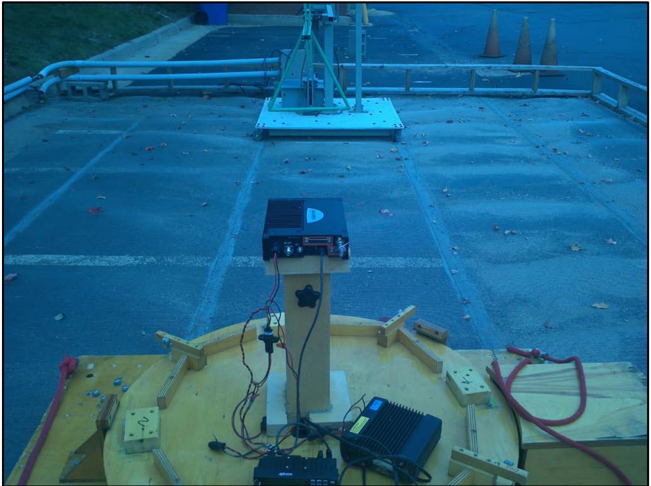
Photograph 2: Radiated Emissions (Spurious/Harmonics) – Back View
