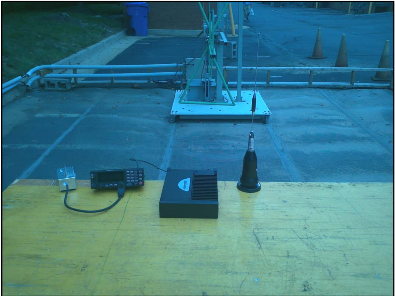
Photograph 3: Radiated Emissions (GNSS) – Front View
