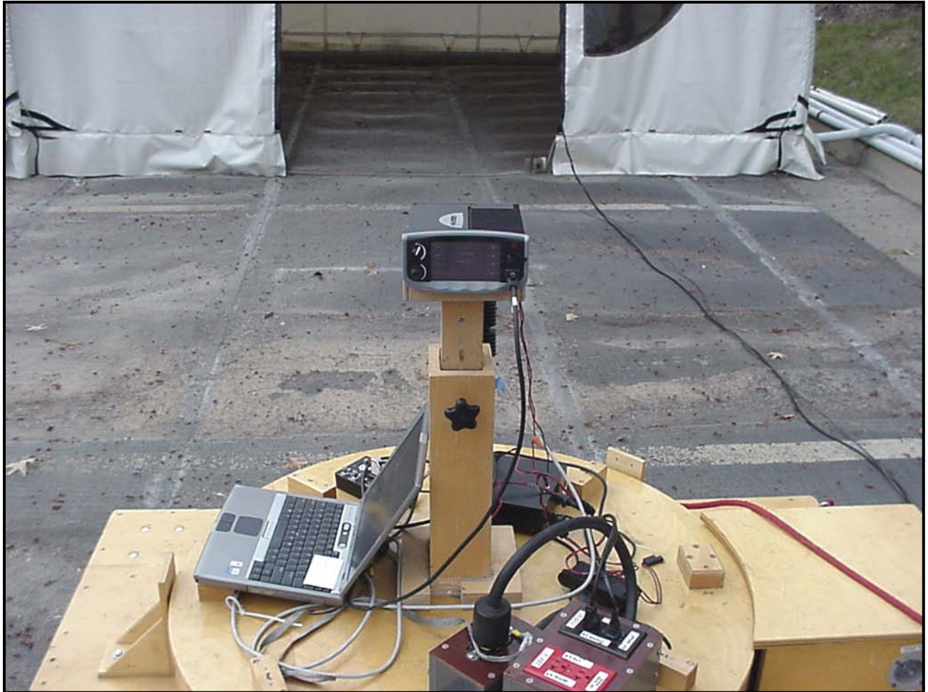
Photograph 3: Radiated Emissions (Spurious/Harmonics) – Front View
