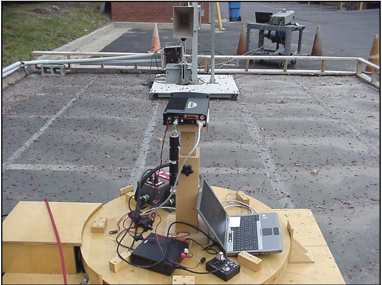
Photograph 4: Radiated Emissions (Spurious/Harmonics) – Back View
