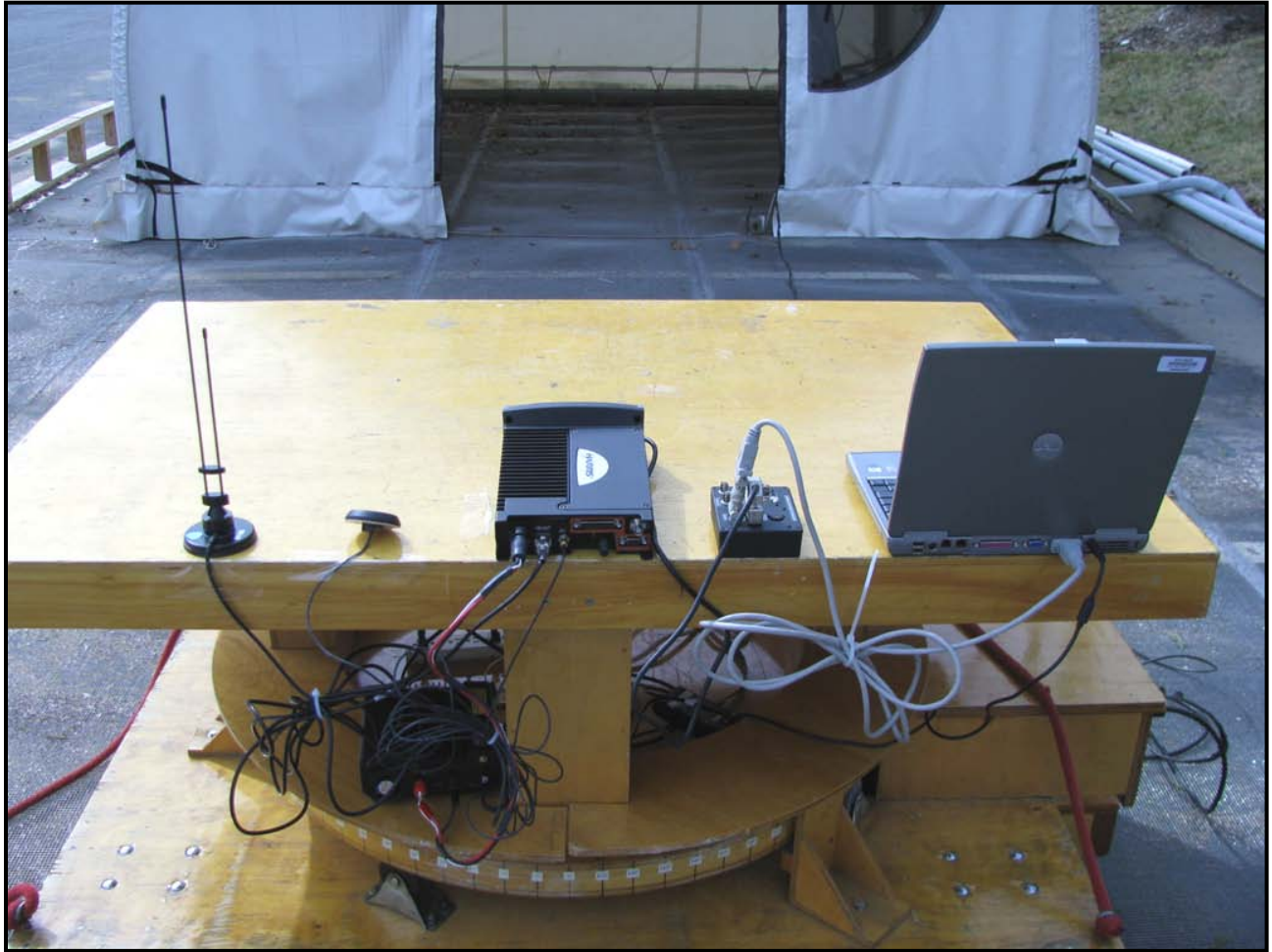
Photograph 6: Radiated Emissions (GNSS) – Back View
